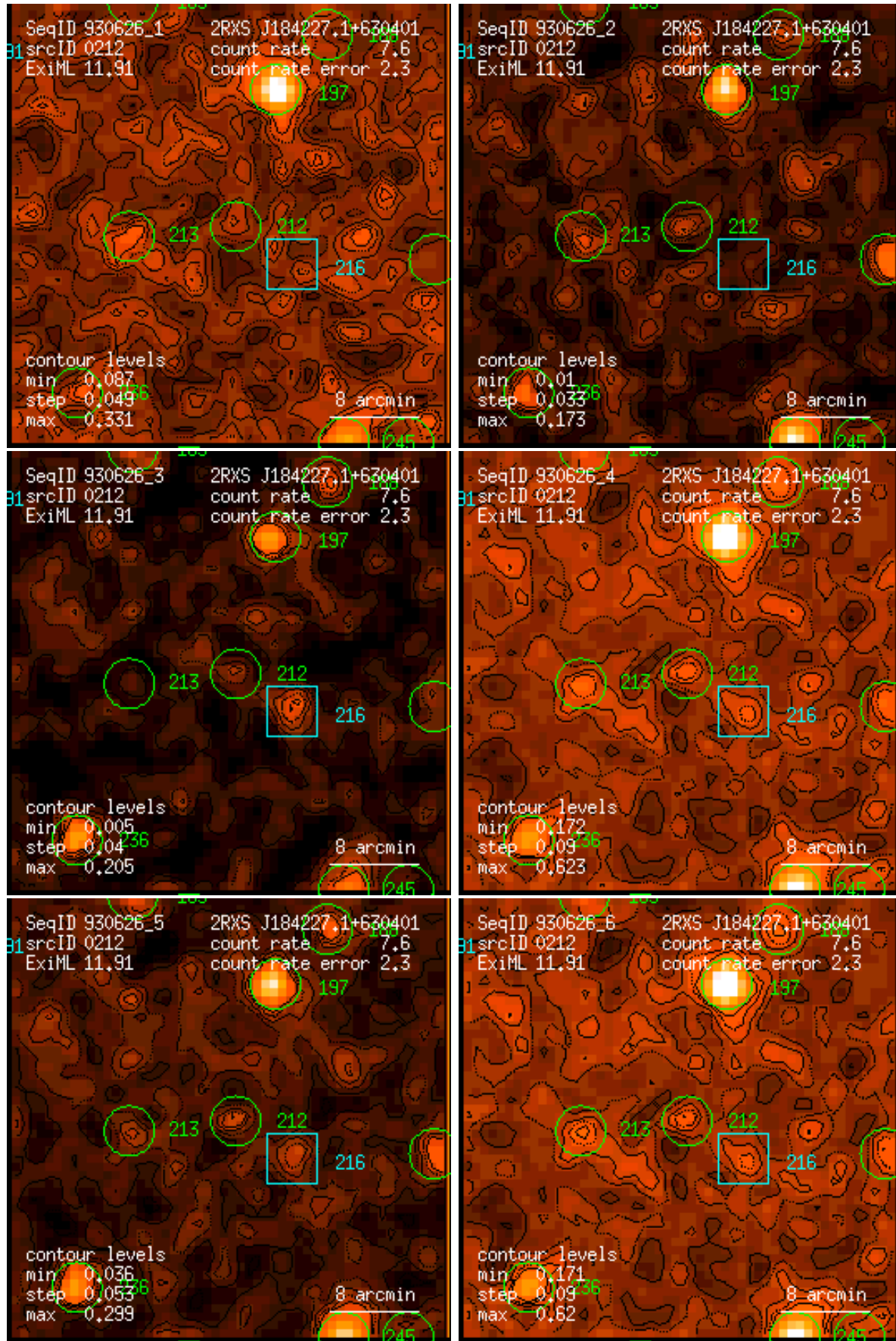
Figure 212: RASS 930626: detection 0212: band rate images, Gaussian filter: (1) PSPC channels 11 – 41, (2) 52 – 90, (3) 91 – 201, (4) 11 – 235, (5) 52 – 201, (6) 11 – 201. Broad band rates in counts/ks. Band rate contour levels in counts/ks/arcmin 2 .
