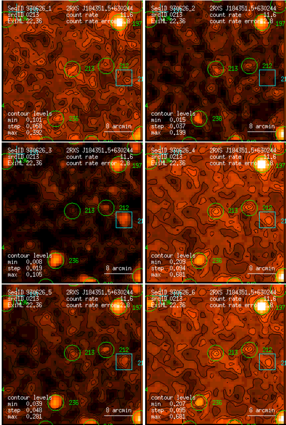
Figure 213: RASS 930626: detection 0213: band rate images, Gaussian filter: (1) PSPC channels 11 – 41, (2) 52 – 90, (3) 91 – 201, (4) 11 – 235, (5) 52 – 201, (6) 11 – 201. Broad band rates in counts/ks. Band rate contour levels in counts/ks/arcmin 2 .
