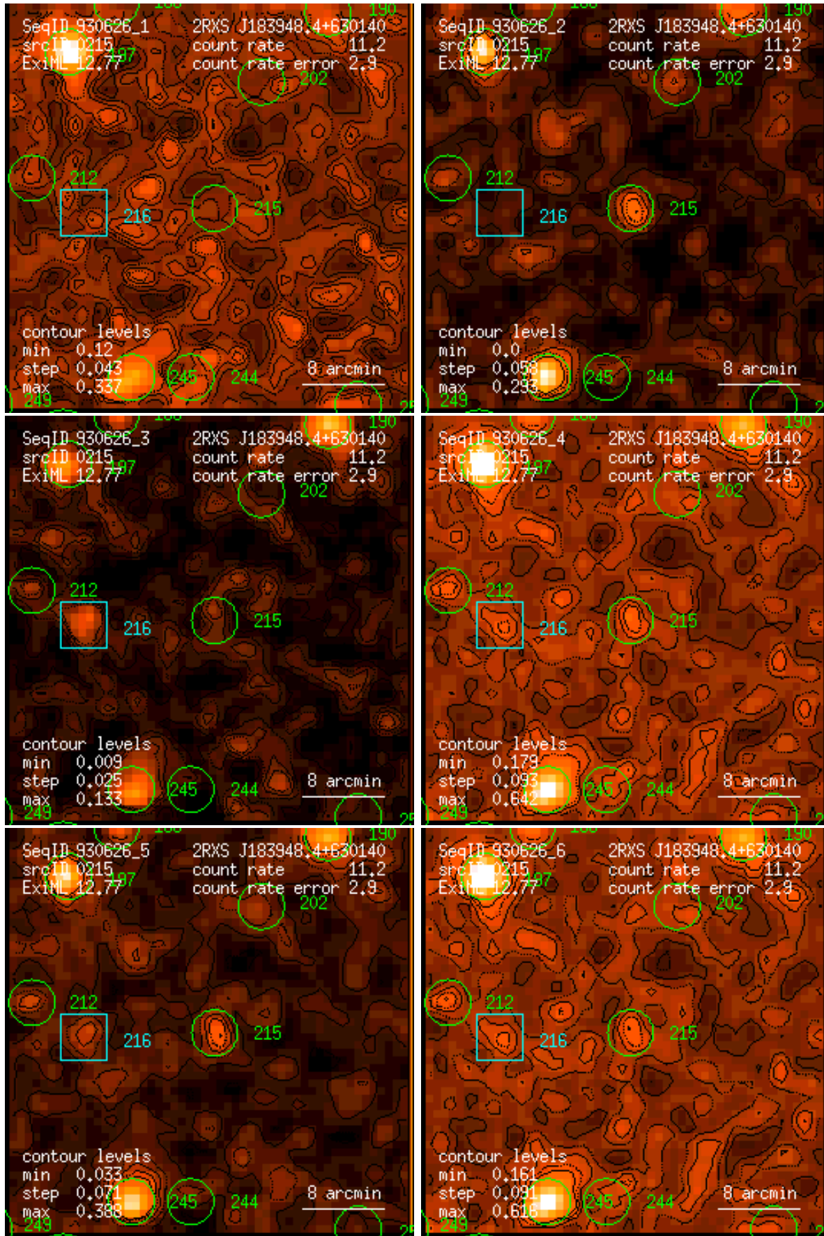
Figure 215: RASS 930626: detection 0215: band rate images, Gaussian filter: (1) PSPC channels 11 – 41, (2) 52 – 90, (3) 91 – 201, (4) 11 – 235, (5) 52 – 201, (6) 11 – 201. Broad band rates in counts/ks. Band rate contour levels in counts/ks/arcmin 2 .
