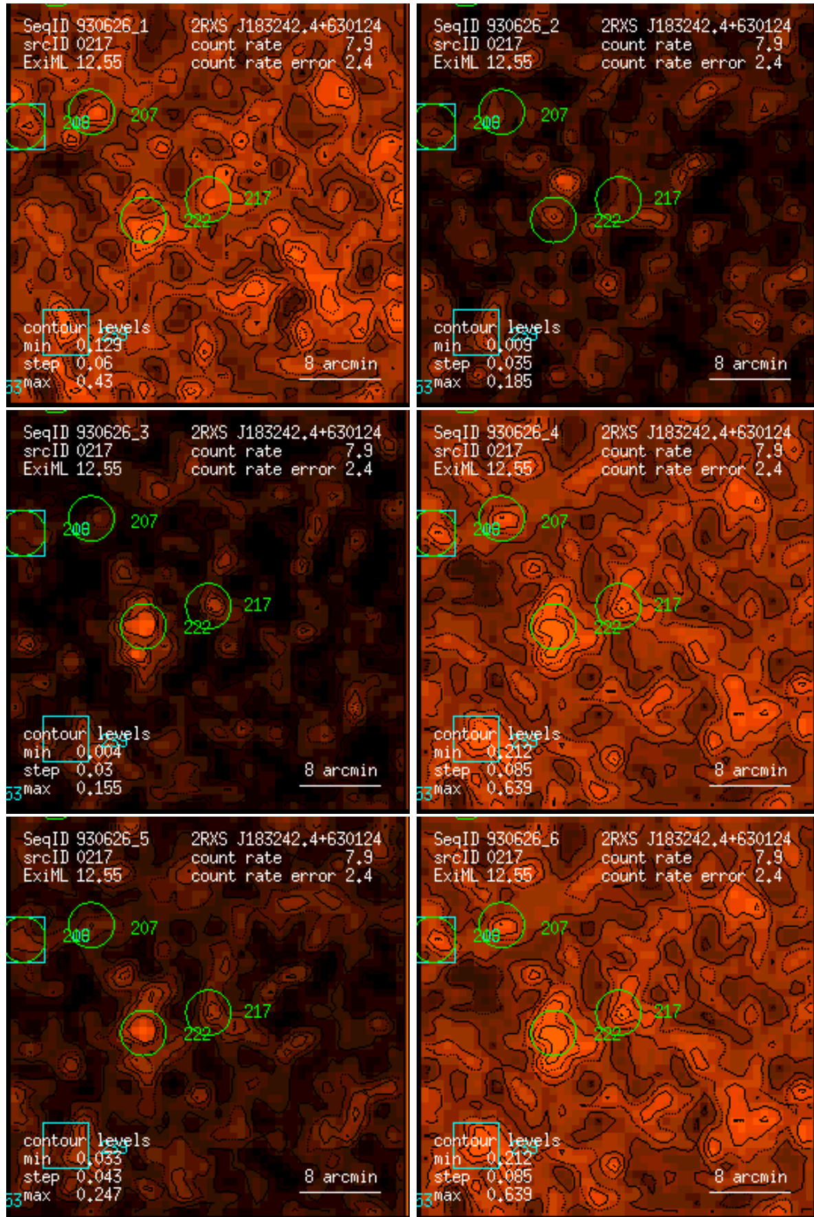
Figure 217: RASS 930626: detection 0217: band rate images, Gaussian filter: (1) PSPC channels 11 – 41, (2) 52 – 90, (3) 91 – 201, (4) 11 – 235, (5) 52 – 201, (6) 11 – 201. Broad band rates in counts/ks. Band rate contour levels in counts/ks/arcmin 2 .
