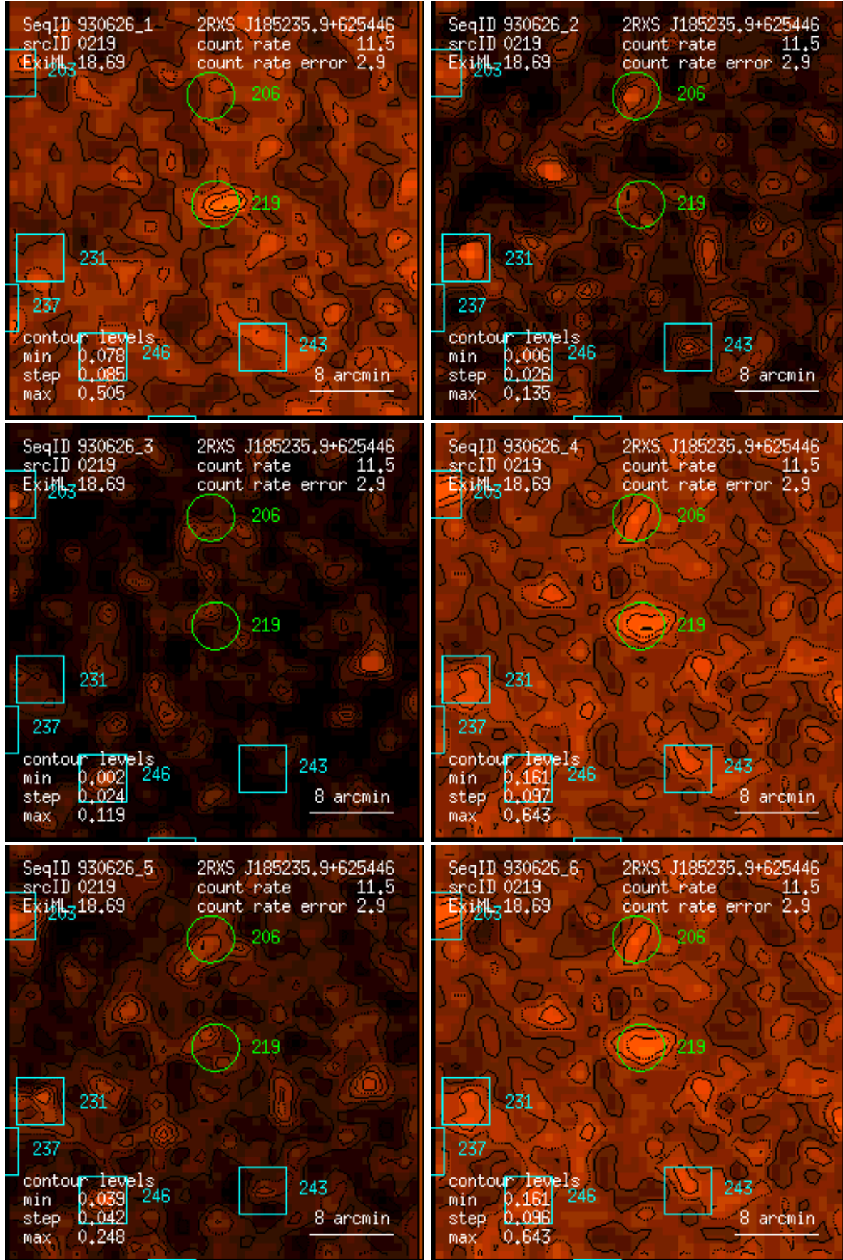
Figure 219: RASS 930626: detection 0219: band rate images, Gaussian filter: (1) PSPC channels 11 – 41, (2) 52 – 90, (3) 91 – 201, (4) 11 – 235, (5) 52 – 201, (6) 11 – 201. Broad band rates in counts/ks. Band rate contour levels in counts/ks/arcmin 2 .
