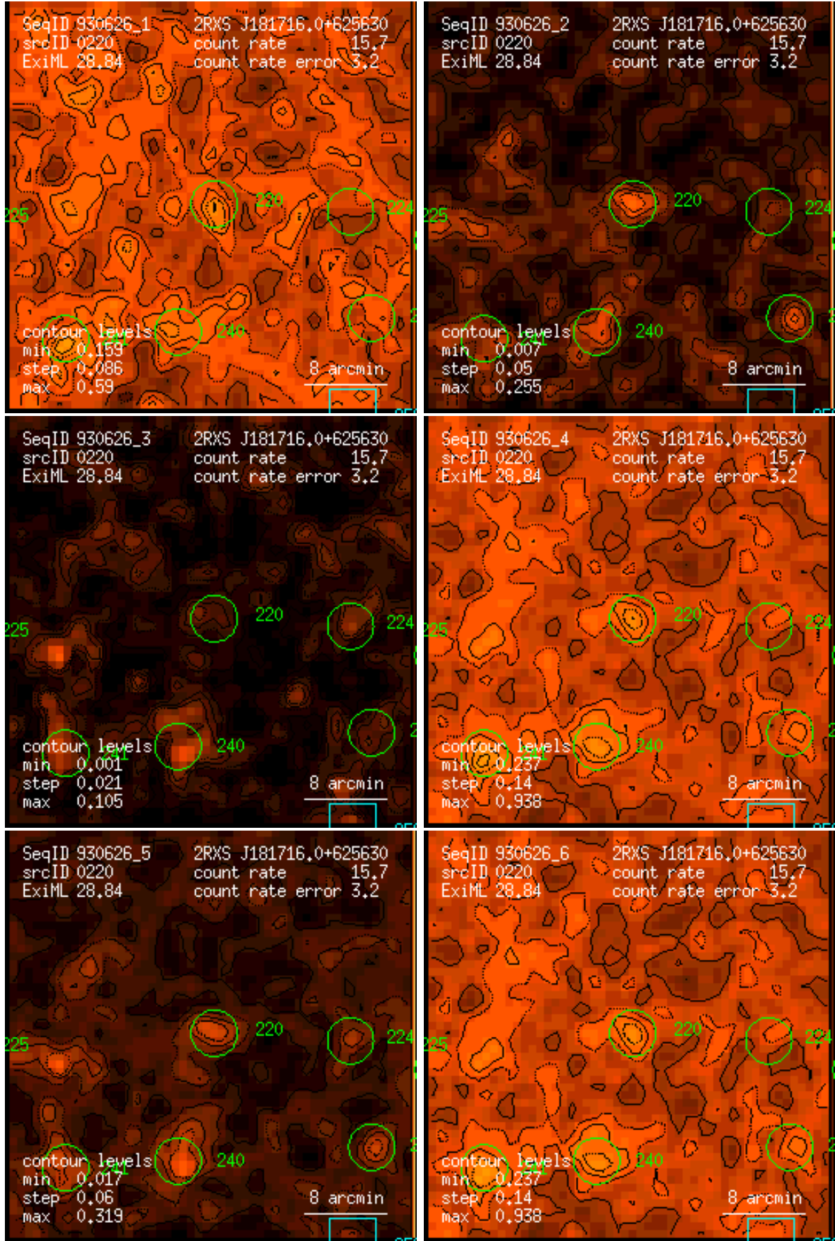
Figure 220: RASS 930626: detection 0220: band rate images, Gaussian filter: (1) PSPC channels 11 – 41, (2) 52 – 90, (3) 91 – 201, (4) 11 – 235, (5) 52 – 201, (6) 11 – 201. Broad band rates in counts/ks. Band rate contour levels in counts/ks/arcmin 2 .
