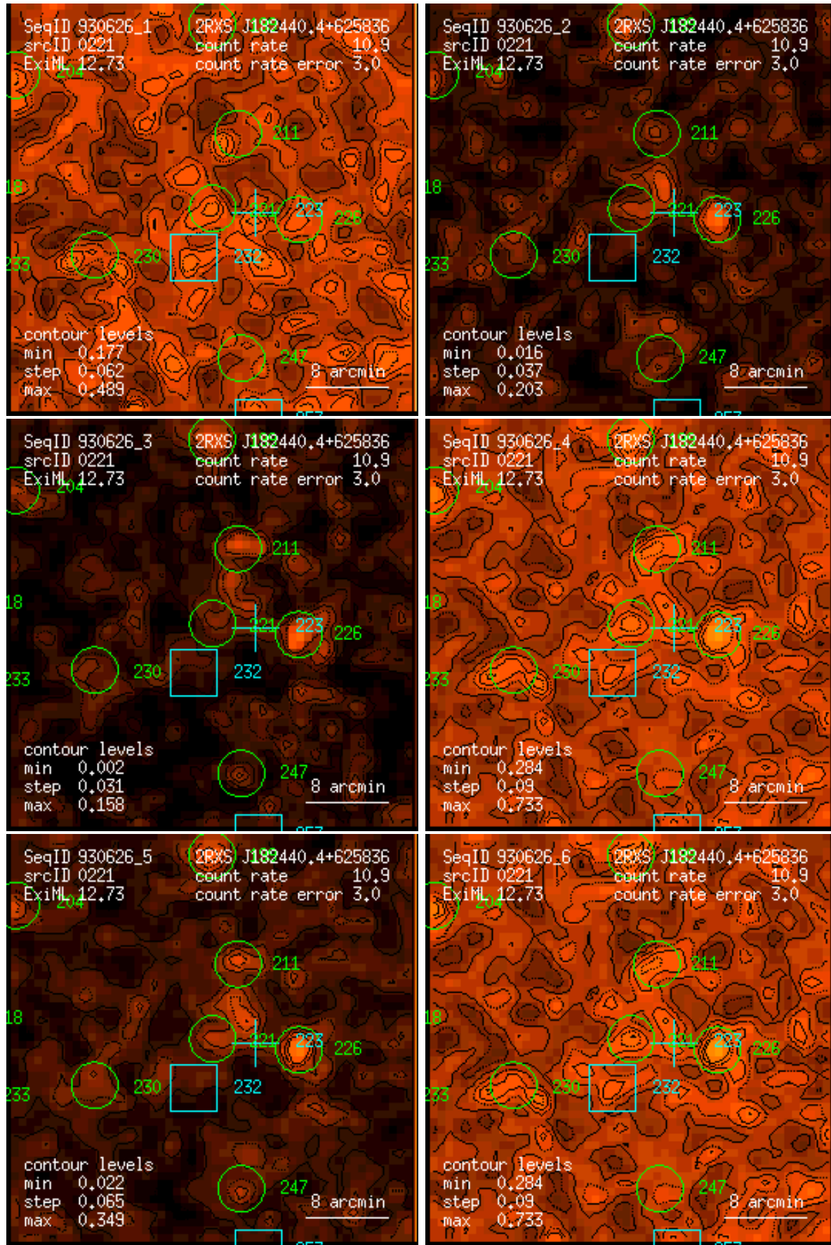
Figure 221: RASS 930626: detection 0221: band rate images, Gaussian filter: (1) PSPC channels 11 – 41, (2) 52 – 90, (3) 91 – 201, (4) 11 – 235, (5) 52 – 201, (6) 11 – 201. Broad band rates in counts/ks. Band rate contour levels in counts/ks/arcmin 2 .
