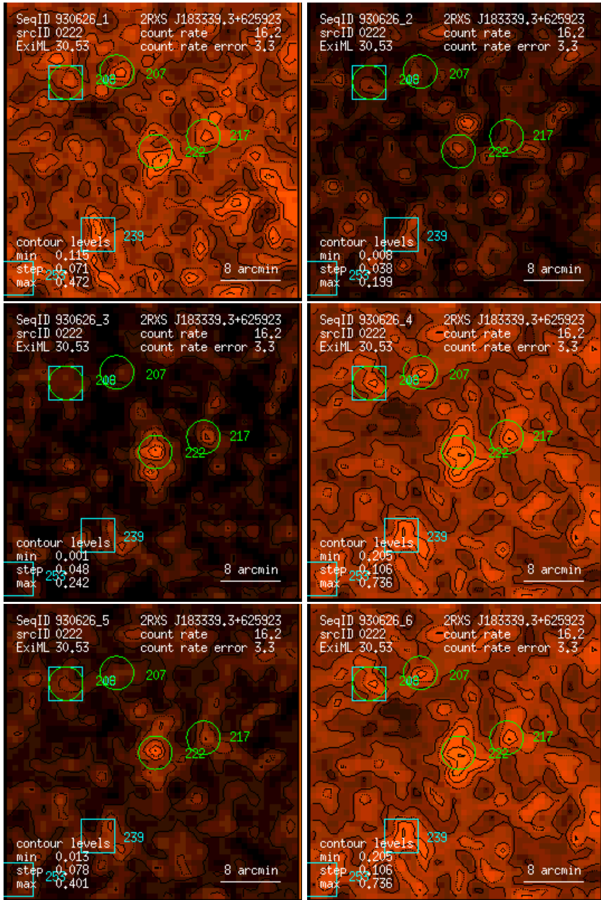
Figure 222: RASS 930626: detection 0222: band rate images, Gaussian filter: (1) PSPC channels 11 – 41, (2) 52 – 90, (3) 91 – 201, (4) 11 – 235, (5) 52 – 201, (6) 11 – 201. Broad band rates in counts/ks. Band rate contour levels in counts/ks/arcmin 2 .
