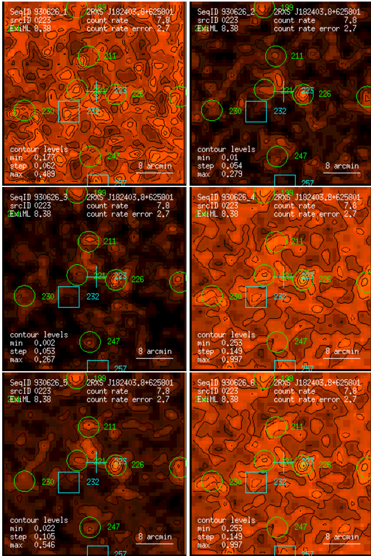
Figure 223: RASS 930626: detection 0223: band rate images, Gaussian filter: (1) PSPC channels 11 – 41, (2) 52 – 90, (3) 91 – 201, (4) 11 – 235, (5) 52 – 201, (6) 11 – 201. Broad band rates in counts/ks. Band rate contour levels in counts/ks/arcmin 2 .
