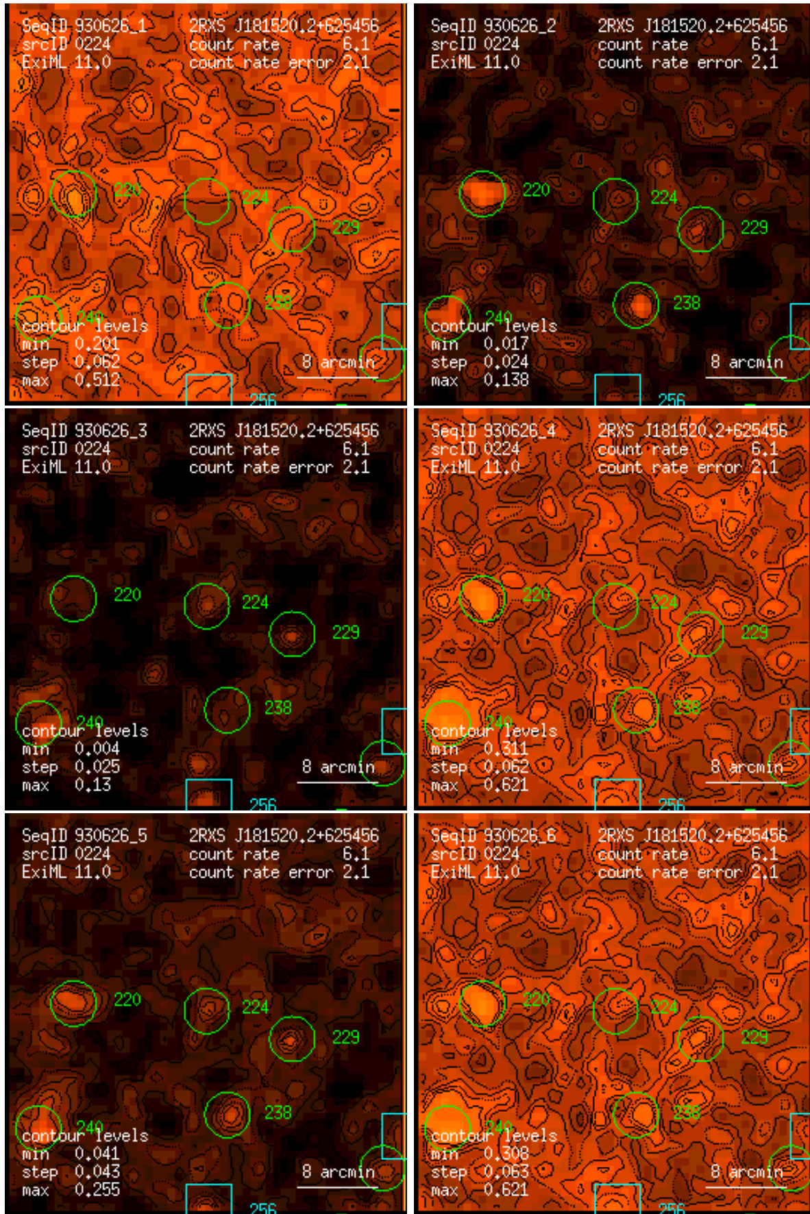
Figure 224: RASS 930626: detection 0224: band rate images, Gaussian filter: (1) PSPC channels 11 – 41, (2) 52 – 90, (3) 91 – 201, (4) 11 – 235, (5) 52 – 201, (6) 11 – 201. Broad band rates in counts/ks. Band rate contour levels in counts/ks/arcmin 2 .
