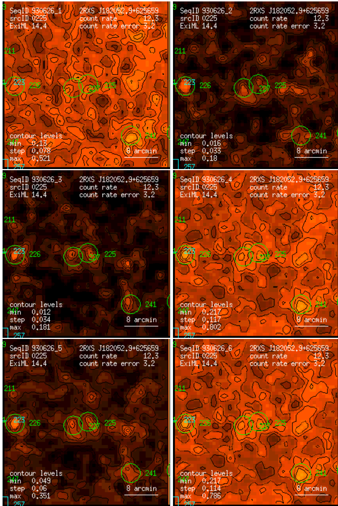
Figure 225: RASS 930626: detection 0225: band rate images, Gaussian filter: (1) PSPC channels 11 – 41, (2) 52 – 90, (3) 91 – 201, (4) 11 – 235, (5) 52 – 201, (6) 11 – 201. Broad band rates in counts/ks. Band rate contour levels in counts/ks/arcmin 2 .
