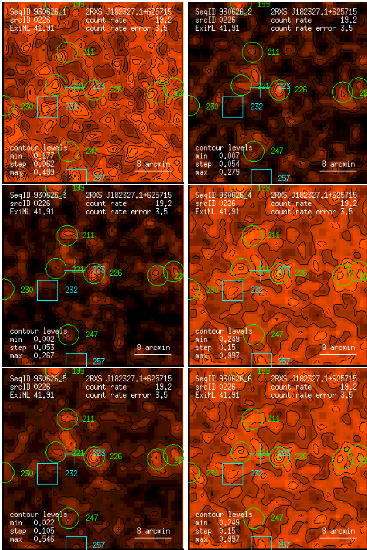
Figure 226: RASS 930626: detection 0226: band rate images, Gaussian filter: (1) PSPC channels 11 – 41, (2) 52 – 90, (3) 91 – 201, (4) 11 – 235, (5) 52 – 201, (6) 11 – 201. Broad band rates in counts/ks. Band rate contour levels in counts/ks/arcmin 2 .
