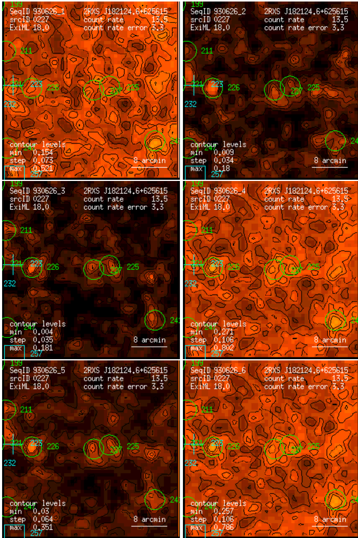
Figure 227: RASS 930626: detection 0227: band rate images, Gaussian filter: (1) PSPC channels 11 – 41, (2) 52 – 90, (3) 91 – 201, (4) 11 – 235, (5) 52 – 201, (6) 11 – 201. Broad band rates in counts/ks. Band rate contour levels in counts/ks/arcmin 2 .
