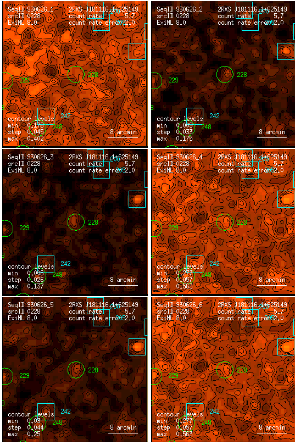
Figure 228: RASS 930626: detection 0228: band rate images, Gaussian filter: (1) PSPC channels 11 – 41, (2) 52 – 90, (3) 91 – 201, (4) 11 – 235, (5) 52 – 201, (6) 11 – 201. Broad band rates in counts/ks. Band rate contour levels in counts/ks/arcmin 2 .
