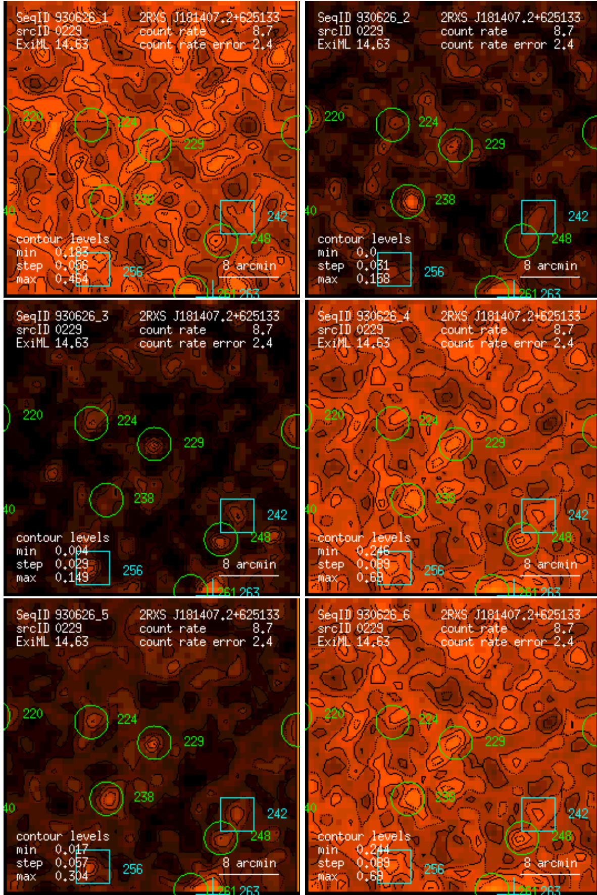
Figure 229: RASS 930626: detection 0229: band rate images, Gaussian filter: (1) PSPC channels 11 – 41, (2) 52 – 90, (3) 91 – 201, (4) 11 – 235, (5) 52 – 201, (6) 11 – 201. Broad band rates in counts/ks. Band rate contour levels in counts/ks/arcmin 2 .
