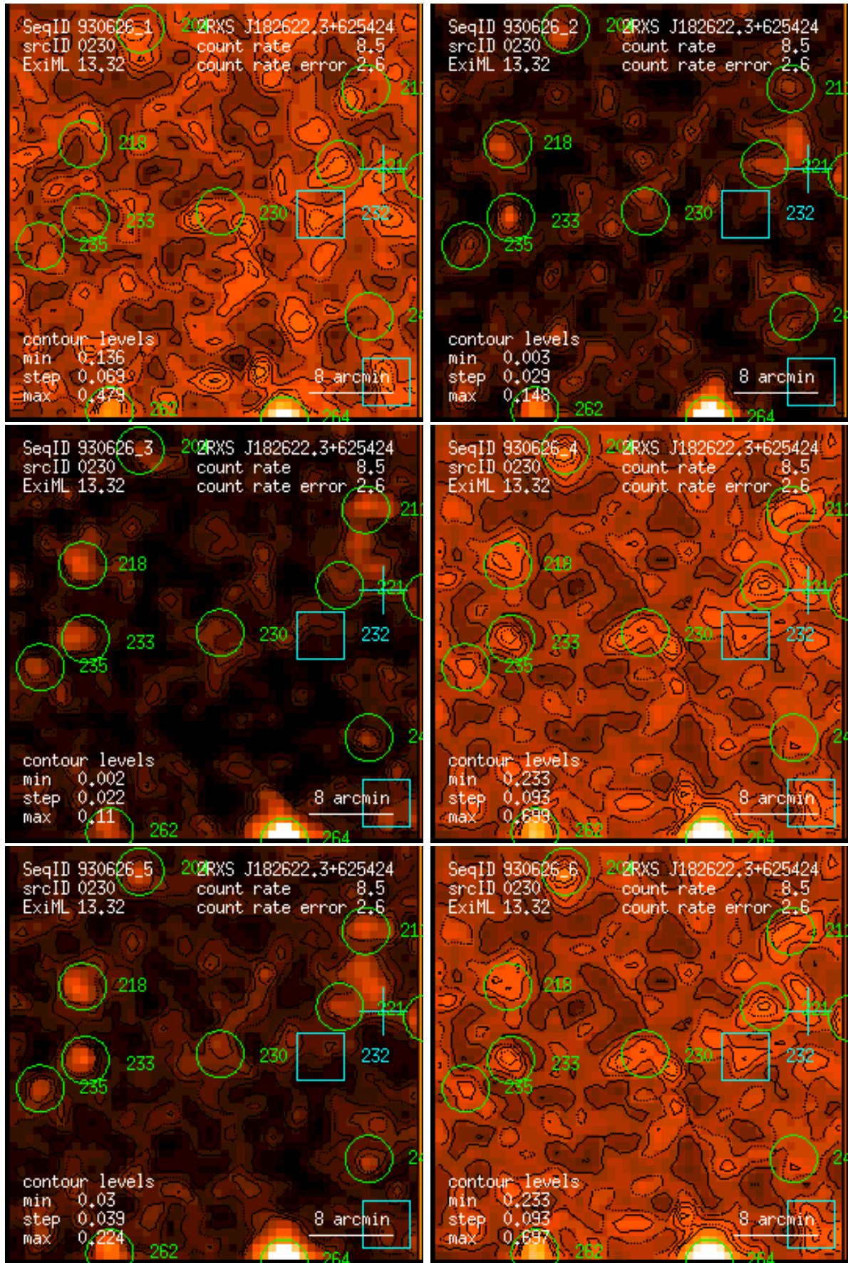
Figure 230: RASS 930626: detection 0230: band rate images, Gaussian filter: (1) PSPC channels 11 – 41, (2) 52 – 90, (3) 91 – 201, (4) 11 – 235, (5) 52 – 201, (6) 11 – 201. Broad band rates in counts/ks. Band rate contour levels in counts/ks/arcmin 2 .
