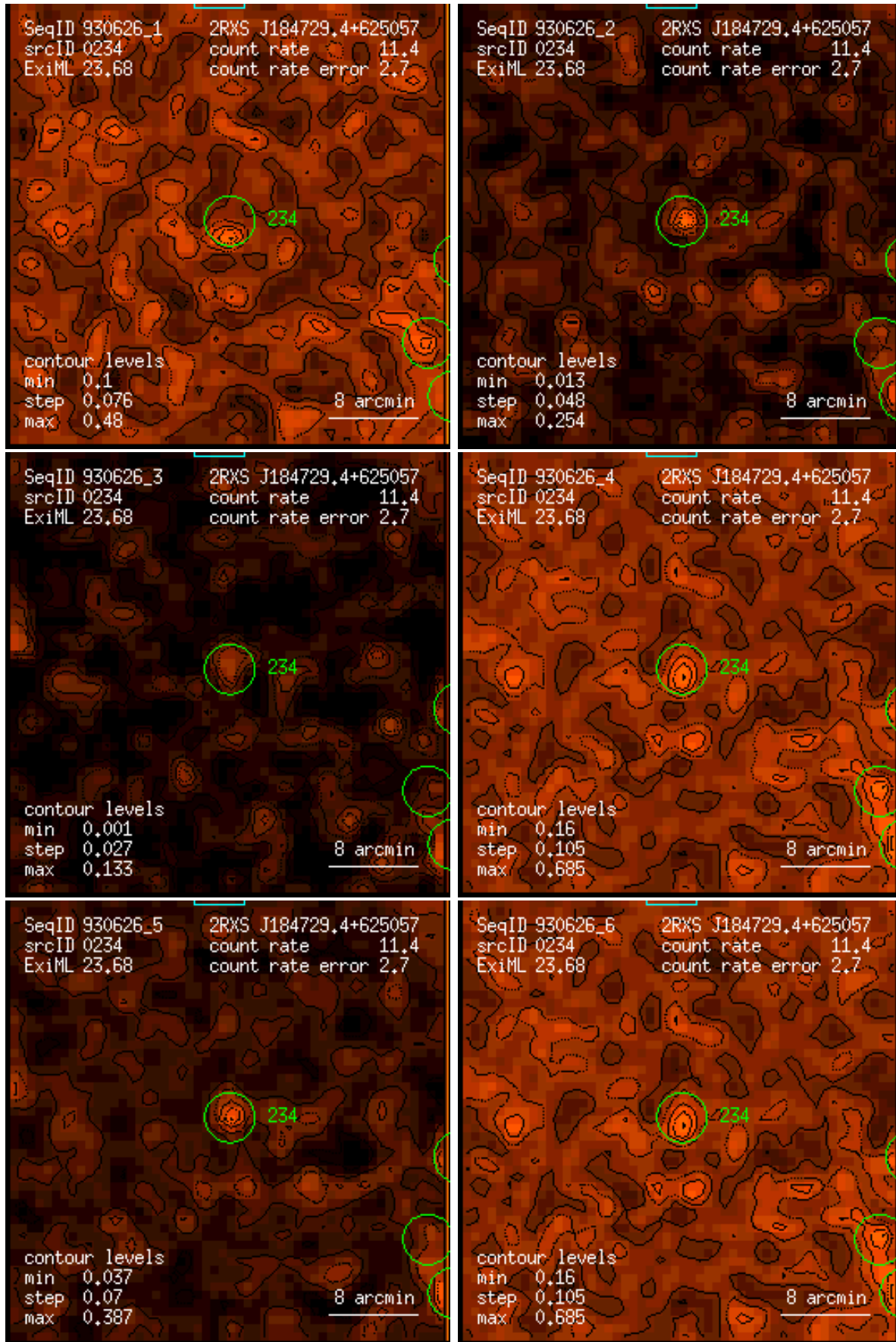
Figure 234: RASS 930626: detection 0234: band rate images, Gaussian filter: (1) PSPC channels 11 – 41, (2) 52 – 90, (3) 91 – 201, (4) 11 – 235, (5) 52 – 201, (6) 11 – 201. Broad band rates in counts/ks. Band rate contour levels in counts/ks/arcmin 2 .
