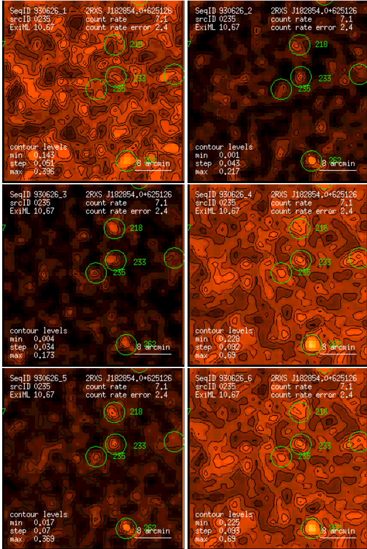
Figure 235: RASS 930626: detection 0235: band rate images, Gaussian filter: (1) PSPC channels 11 – 41, (2) 52 – 90, (3) 91 – 201, (4) 11 – 235, (5) 52 – 201, (6) 11 – 201. Broad band rates in counts/ks. Band rate contour levels in counts/ks/arcmin 2 .
