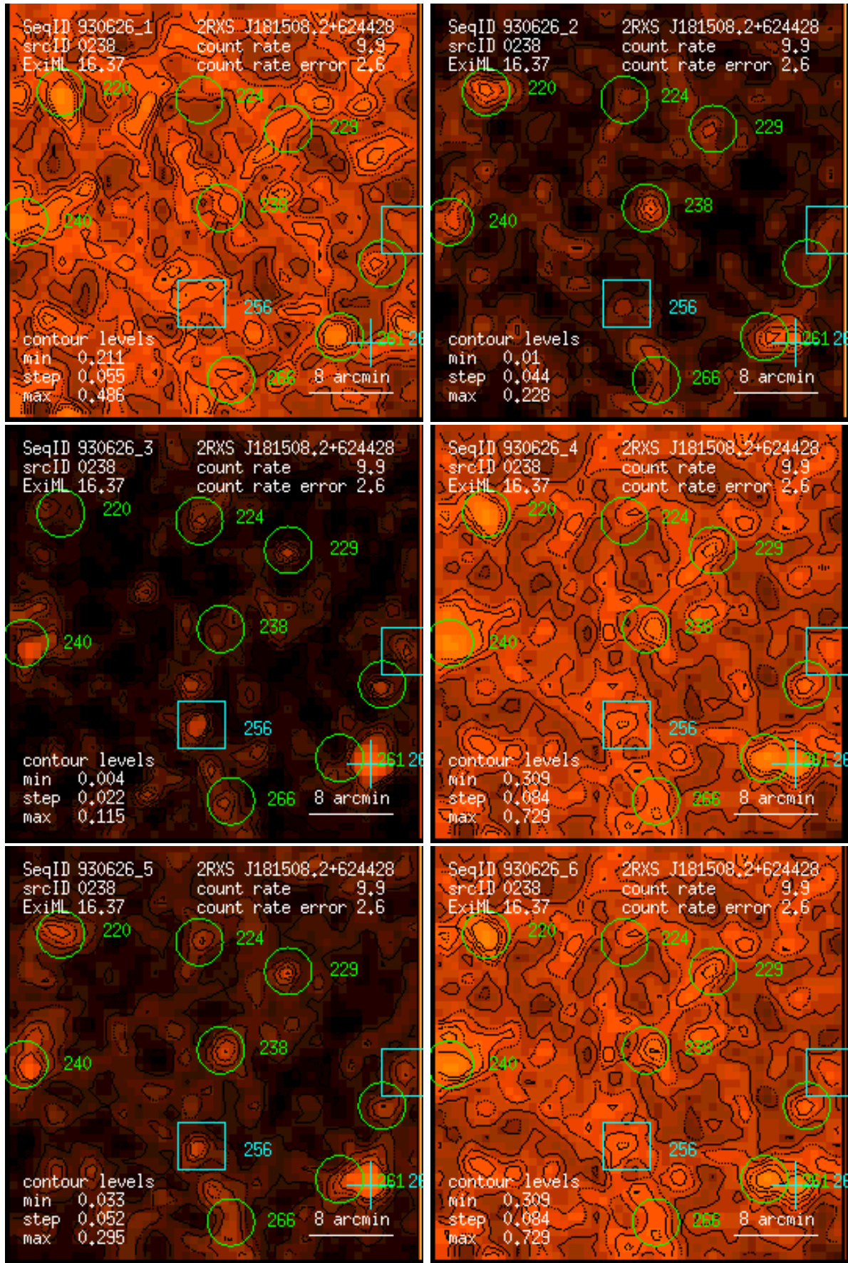
Figure 238: RASS 930626: detection 0238: band rate images, Gaussian filter: (1) PSPC channels 11 – 41, (2) 52 – 90, (3) 91 – 201, (4) 11 – 235, (5) 52 – 201, (6) 11 – 201. Broad band rates in counts/ks. Band rate contour levels in counts/ks/arcmin 2 .
