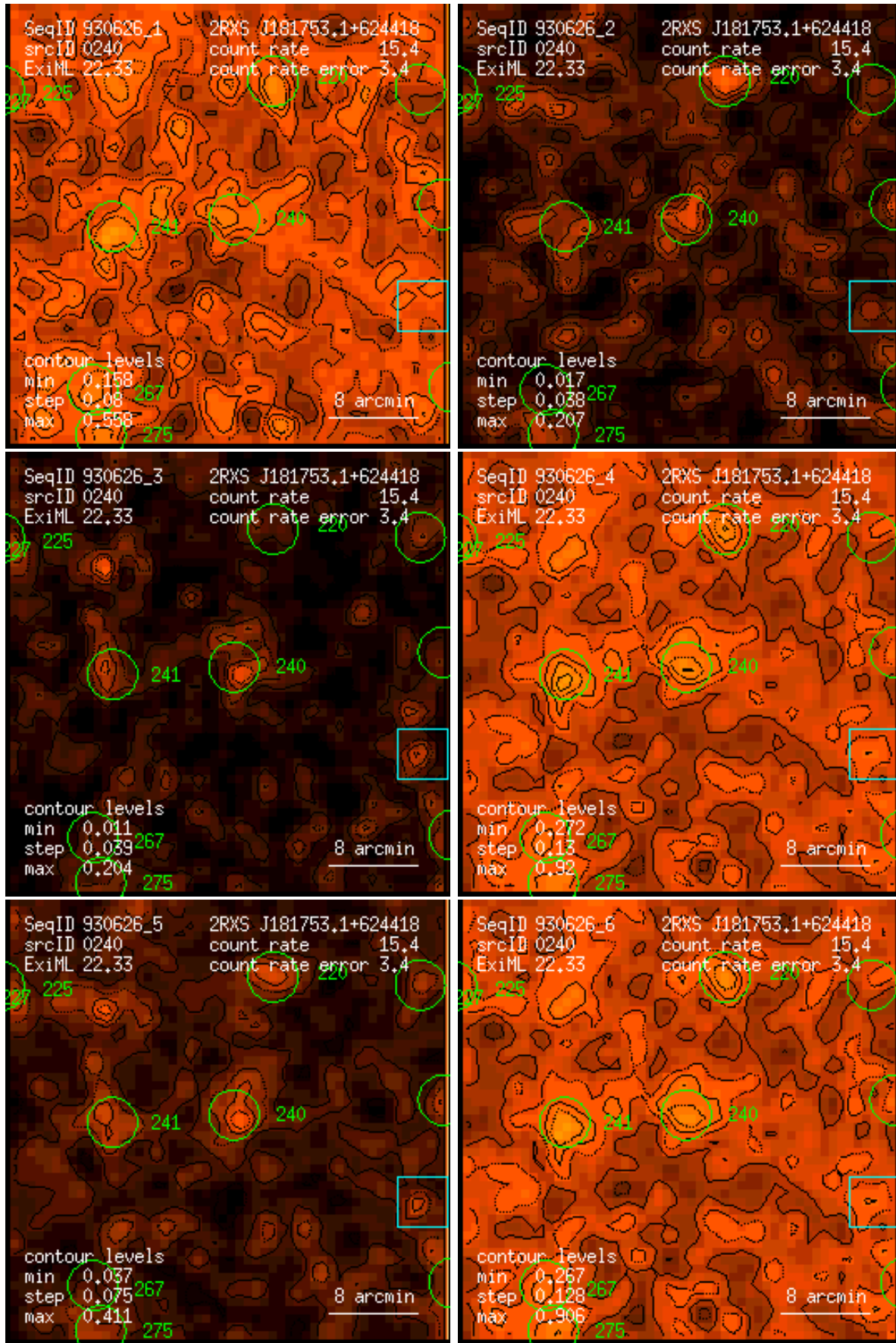
Figure 240: RASS 930626: detection 0240: band rate images, Gaussian filter: (1) PSPC channels 11 – 41, (2) 52 – 90, (3) 91 – 201, (4) 11 – 235, (5) 52 – 201, (6) 11 – 201. Broad band rates in counts/ks. Band rate contour levels in counts/ks/arcmin 2 .
