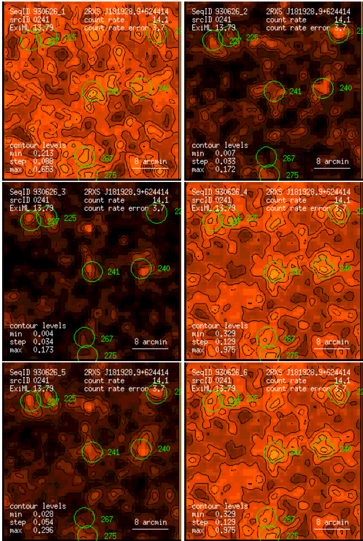
Figure 241: RASS 930626: detection 0241: band rate images, Gaussian filter: (1) PSPC channels 11 – 41, (2) 52 – 90, (3) 91 – 201, (4) 11 – 235, (5) 52 – 201, (6) 11 – 201. Broad band rates in counts/ks. Band rate contour levels in counts/ks/arcmin 2 .
