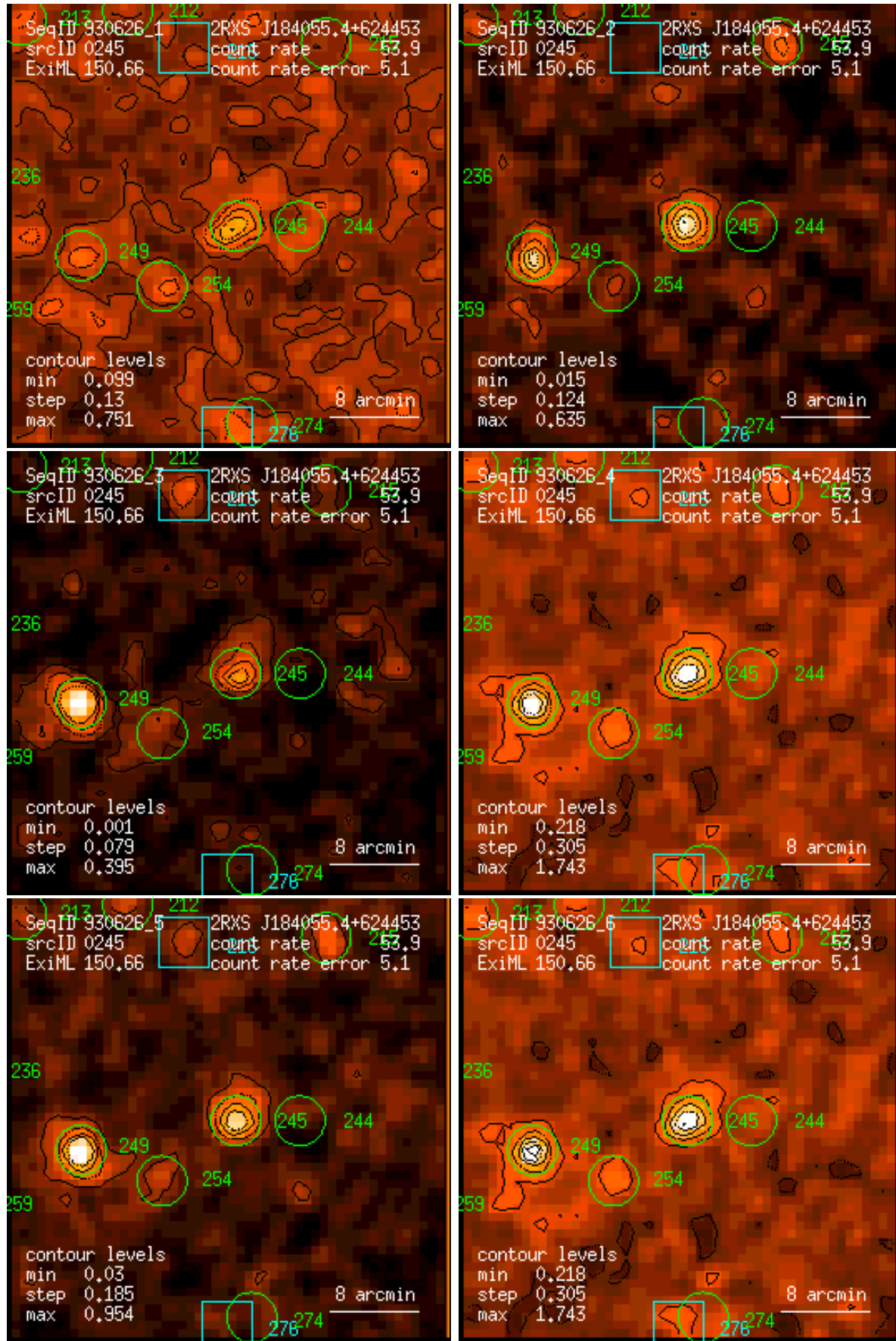
Figure 245: RASS 930626: detection 0245: band rate images, Gaussian filter: (1) PSPC channels 11 – 41, (2) 52 – 90, (3) 91 – 201, (4) 11 – 235, (5) 52 – 201, (6) 11 – 201. Broad band rates in counts/ks. Band rate contour levels in counts/ks/arcmin 2 .
