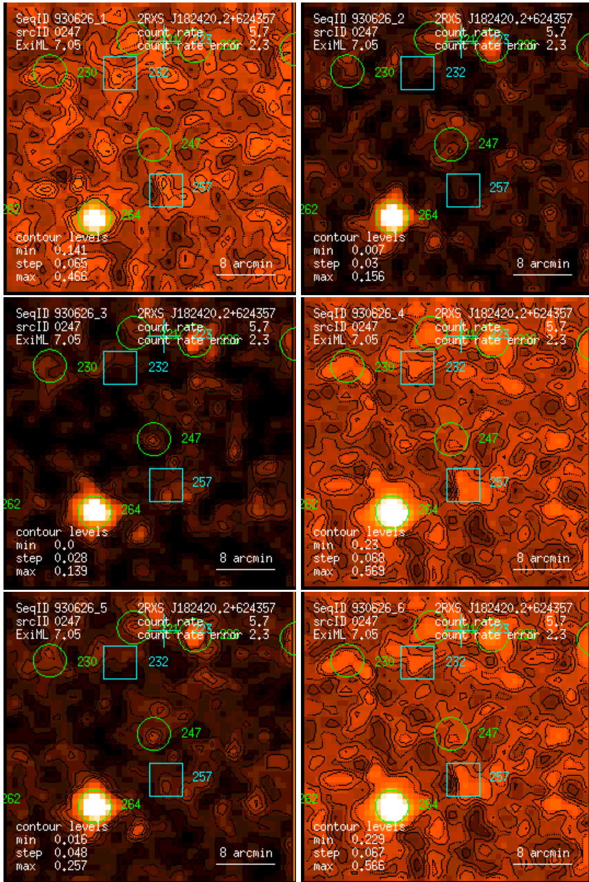
Figure 247: RASS 930626: detection 0247: band rate images, Gaussian filter: (1) PSPC channels 11 – 41, (2) 52 – 90, (3) 91 – 201, (4) 11 – 235, (5) 52 – 201, (6) 11 – 201. Broad band rates in counts/ks. Band rate contour levels in counts/ks/arcmin 2 .
