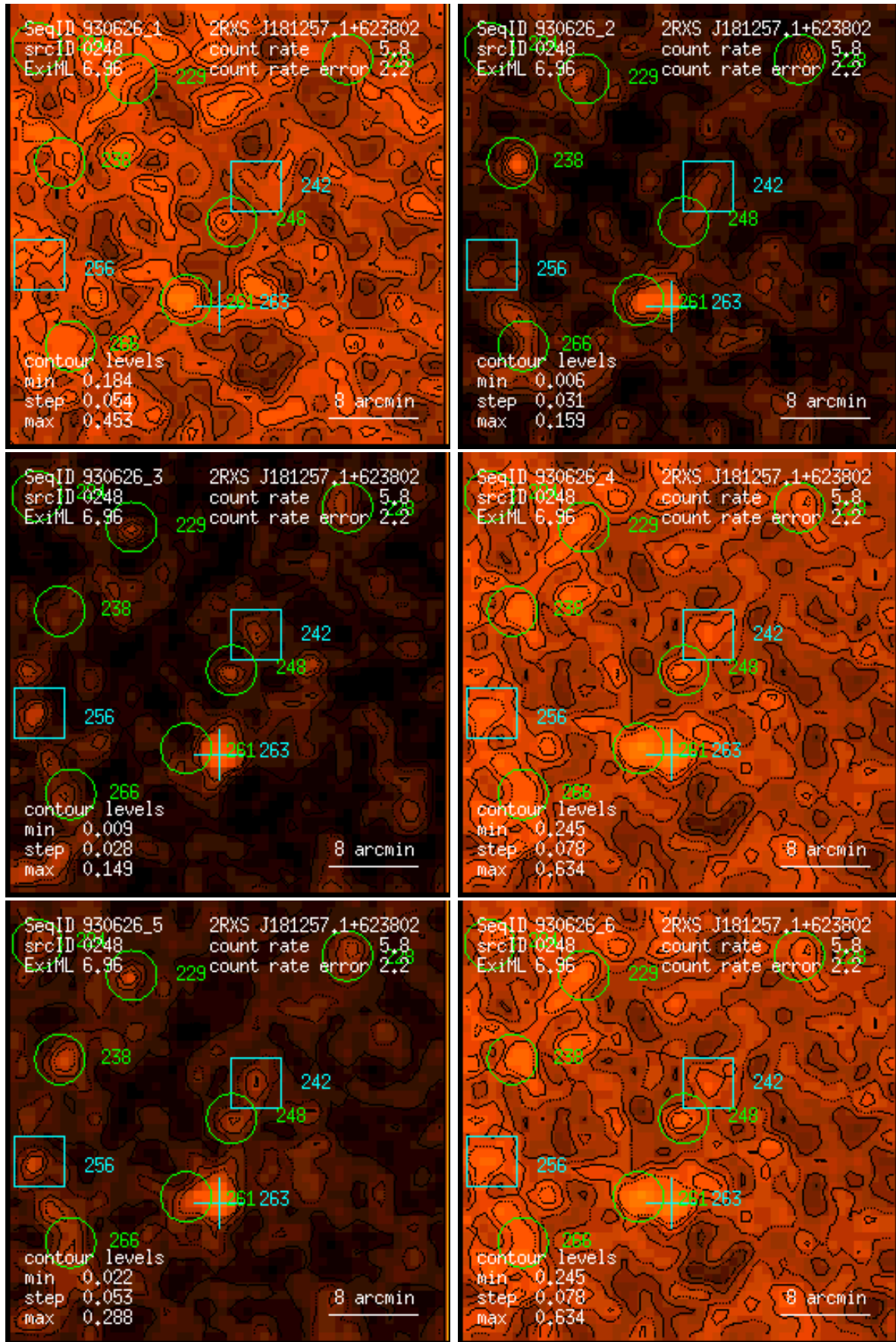
Figure 248: RASS 930626: detection 0248: band rate images, Gaussian filter: (1) PSPC channels 11 – 41, (2) 52 – 90, (3) 91 – 201, (4) 11 – 235, (5) 52 – 201, (6) 11 – 201. Broad band rates in counts/ks. Band rate contour levels in counts/ks/arcmin 2 .
