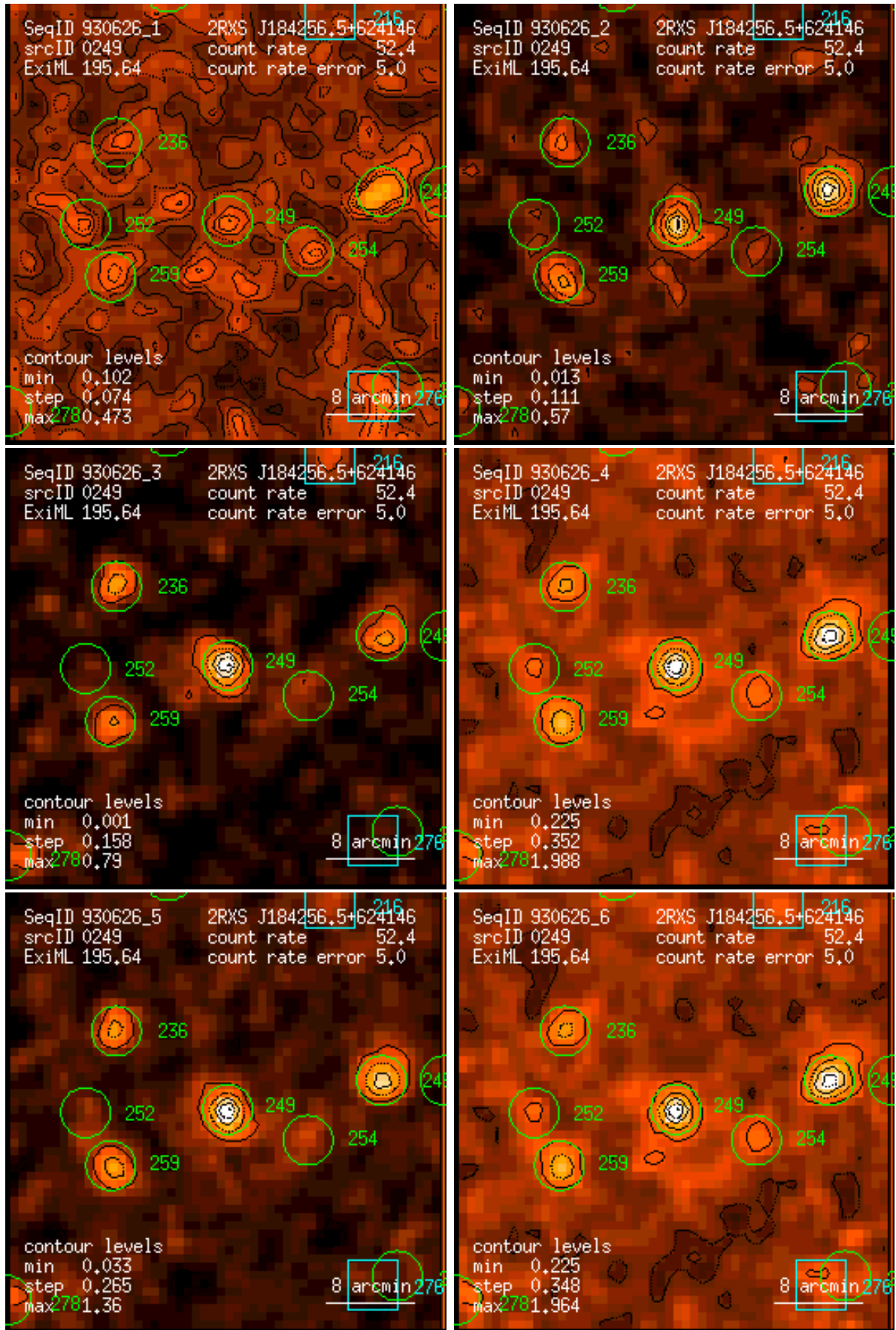
Figure 249: RASS 930626: detection 0249: band rate images, Gaussian filter: (1) PSPC channels 11 – 41, (2) 52 – 90, (3) 91 – 201, (4) 11 – 235, (5) 52 – 201, (6) 11 – 201. Broad band rates in counts/ks. Band rate contour levels in counts/ks/arcmin 2 .
