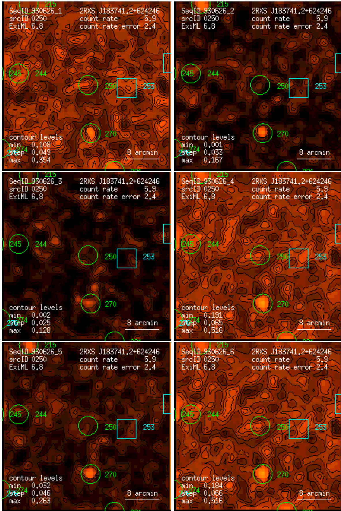
Figure 250: RASS 930626: detection 0250: band rate images, Gaussian filter: (1) PSPC channels 11 – 41, (2) 52 – 90, (3) 91 – 201, (4) 11 – 235, (5) 52 – 201, (6) 11 – 201. Broad band rates in counts/ks. Band rate contour levels in counts/ks/arcmin 2 .
