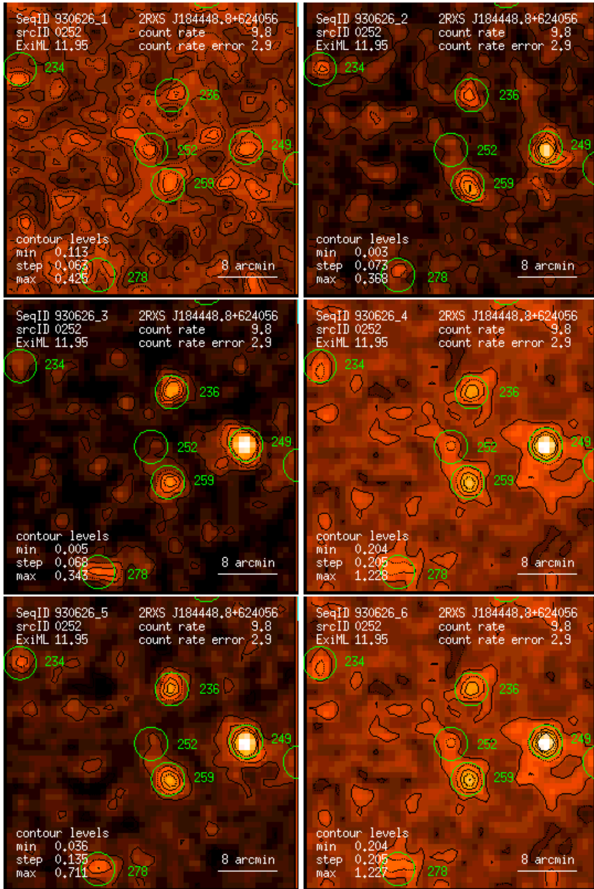
Figure 252: RASS 930626: detection 0252: band rate images, Gaussian filter: (1) PSPC channels 11 – 41, (2) 52 – 90, (3) 91 – 201, (4) 11 – 235, (5) 52 – 201, (6) 11 – 201. Broad band rates in counts/ks. Band rate contour levels in counts/ks/arcmin 2 .
