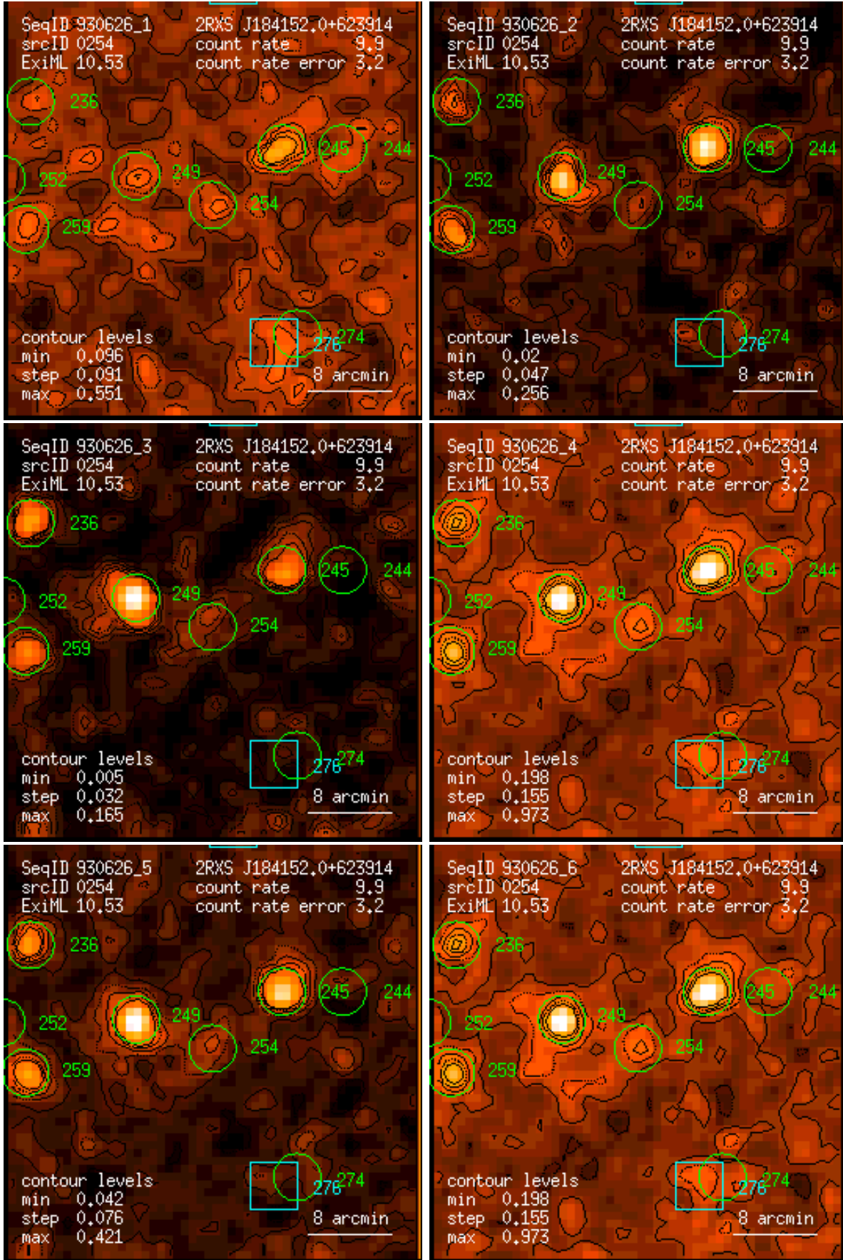
Figure 254: RASS 930626: detection 0254: band rate images, Gaussian filter: (1) PSPC channels 11 – 41, (2) 52 – 90, (3) 91 – 201, (4) 11 – 235, (5) 52 – 201, (6) 11 – 201. Broad band rates in counts/ks. Band rate contour levels in counts/ks/arcmin 2 .
