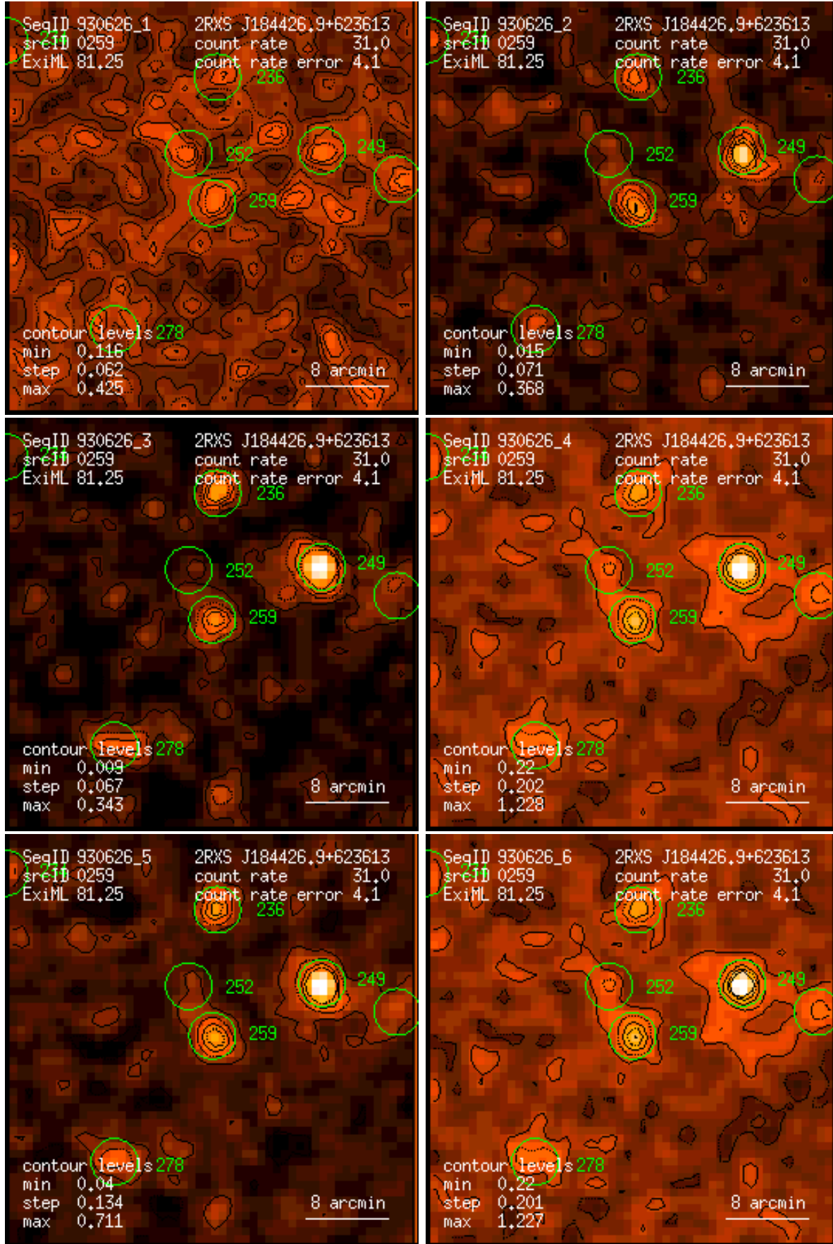
Figure 259: RASS 930626: detection 0259: band rate images, Gaussian filter: (1) PSPC channels 11 – 41, (2) 52 – 90, (3) 91 – 201, (4) 11 – 235, (5) 52 – 201, (6) 11 – 201. Broad band rates in counts/ks. Band rate contour levels in counts/ks/arcmin 2 .
