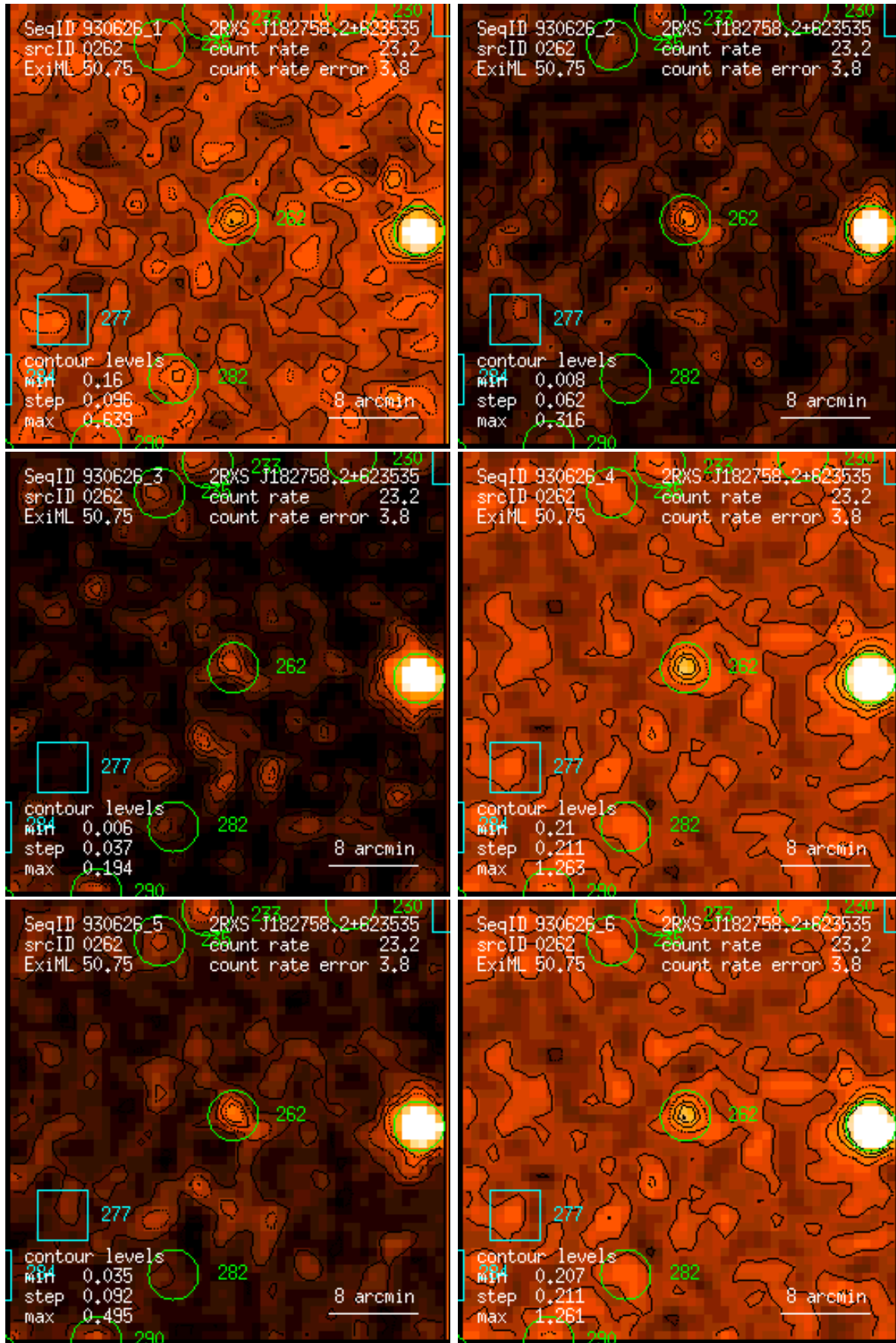
Figure 262: RASS 930626: detection 0262: band rate images, Gaussian filter: (1) PSPC channels 11 – 41, (2) 52 – 90, (3) 91 – 201, (4) 11 – 235, (5) 52 – 201, (6) 11 – 201. Broad band rates in counts/ks. Band rate contour levels in counts/ks/arcmin 2 .
