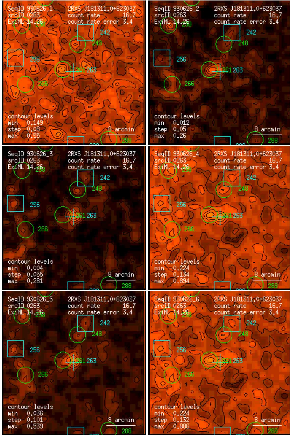
Figure 263: RASS 930626: detection 0263: band rate images, Gaussian filter: (1) PSPC channels 11 – 41, (2) 52 – 90, (3) 91 – 201, (4) 11 – 235, (5) 52 – 201, (6) 11 – 201. Broad band rates in counts/ks. Band rate contour levels in counts/ks/arcmin 2 .
