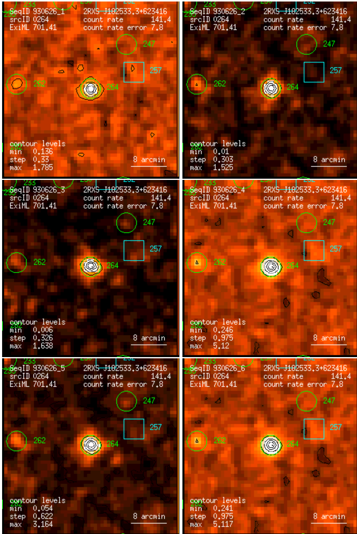
Figure 264: RASS 930626: detection 0264: band rate images, Gaussian filter: (1) PSPC channels 11 – 41, (2) 52 – 90, (3) 91 – 201, (4) 11 – 235, (5) 52 – 201, (6) 11 – 201. Broad band rates in counts/ks. Band rate contour levels in counts/ks/arcmin 2 .
