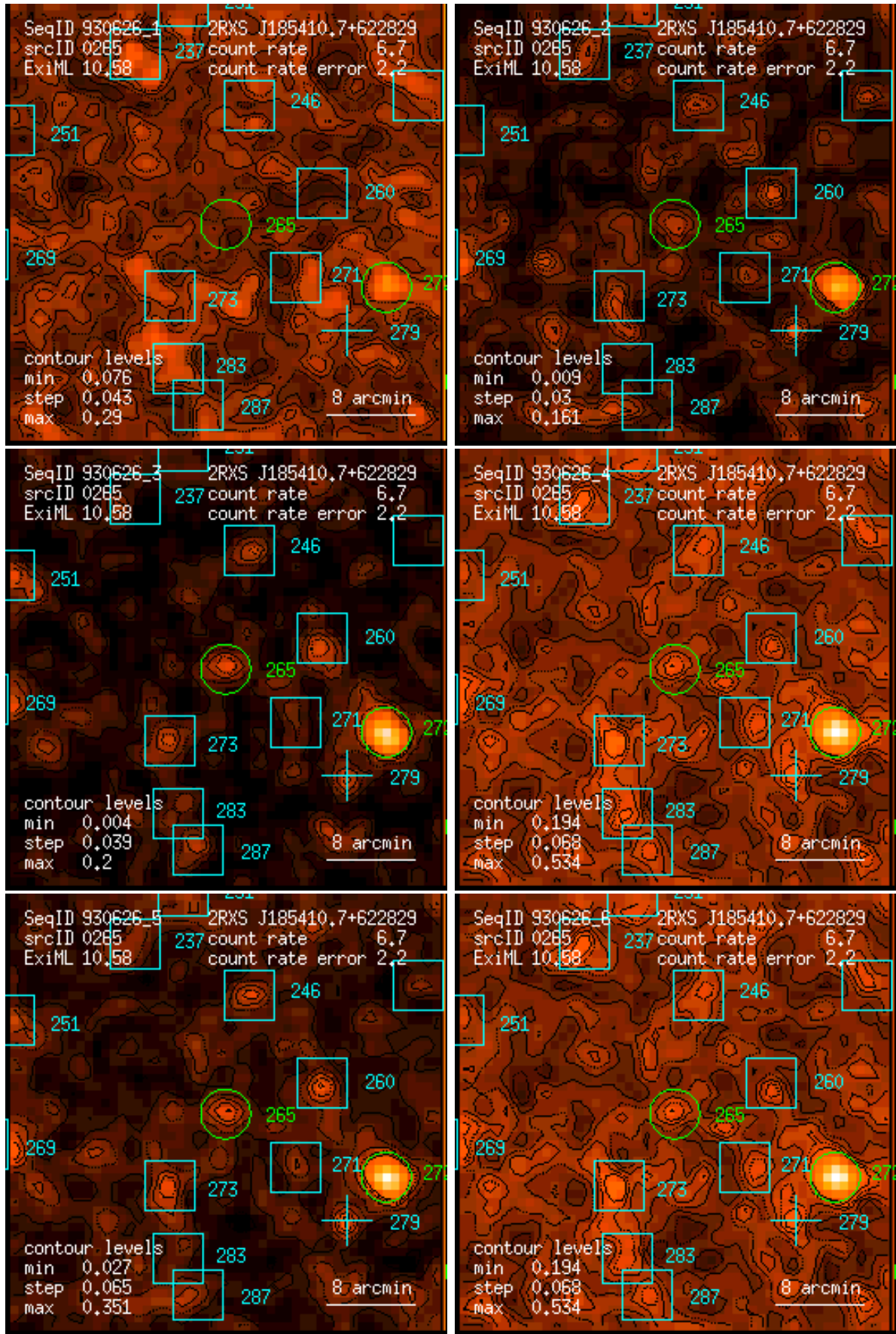
Figure 265: RASS 930626: detection 0265: band rate images, Gaussian filter: (1) PSPC channels 11 – 41, (2) 52 – 90, (3) 91 – 201, (4) 11 – 235, (5) 52 – 201, (6) 11 – 201. Broad band rates in counts/ks. Band rate contour levels in counts/ks/arcmin 2 .
