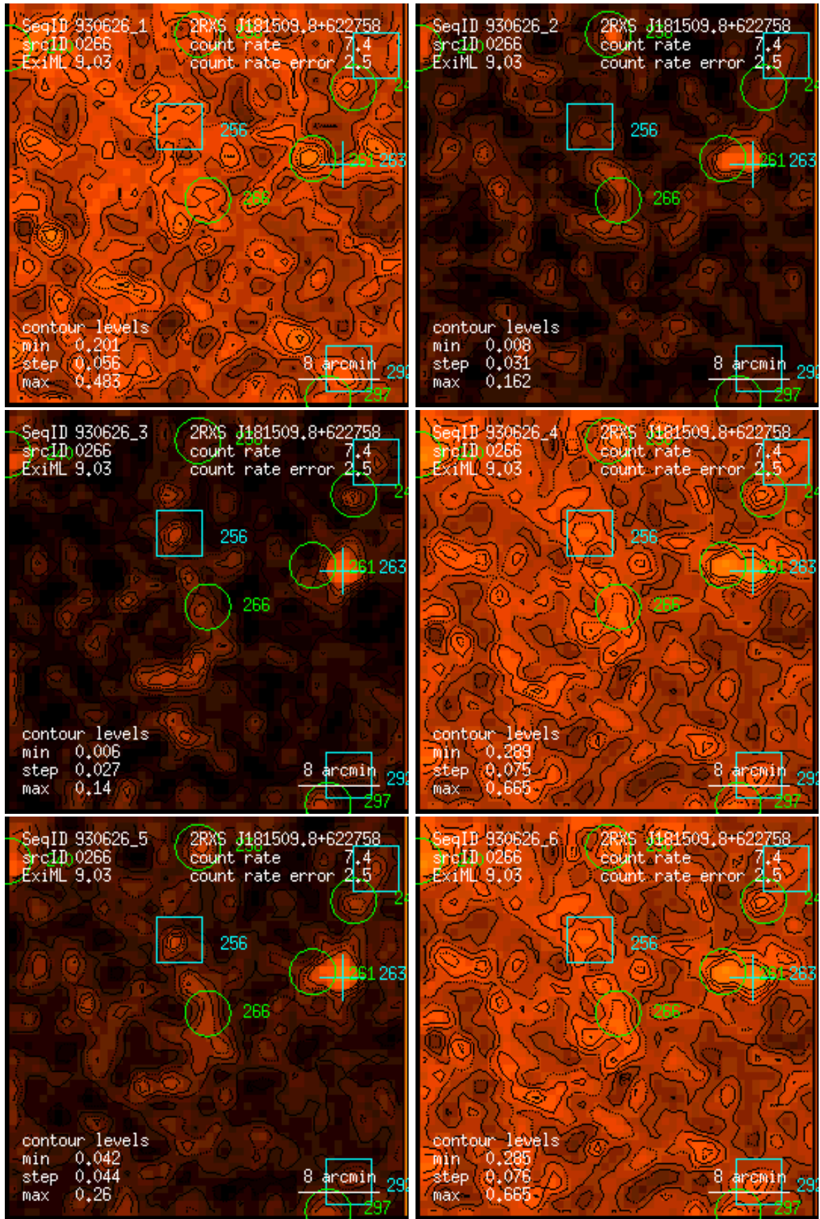
Figure 266: RASS 930626: detection 0266: band rate images, Gaussian filter: (1) PSPC channels 11 – 41, (2) 52 – 90, (3) 91 – 201, (4) 11 – 235, (5) 52 – 201, (6) 11 – 201. Broad band rates in counts/ks. Band rate contour levels in counts/ks/arcmin 2 .
