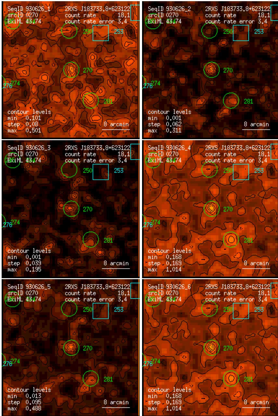
Figure 270: RASS 930626: detection 0270: band rate images, Gaussian filter: (1) PSPC channels 11 – 41, (2) 52 – 90, (3) 91 – 201, (4) 11 – 235, (5) 52 – 201, (6) 11 – 201. Broad band rates in counts/ks. Band rate contour levels in counts/ks/arcmin 2 .
