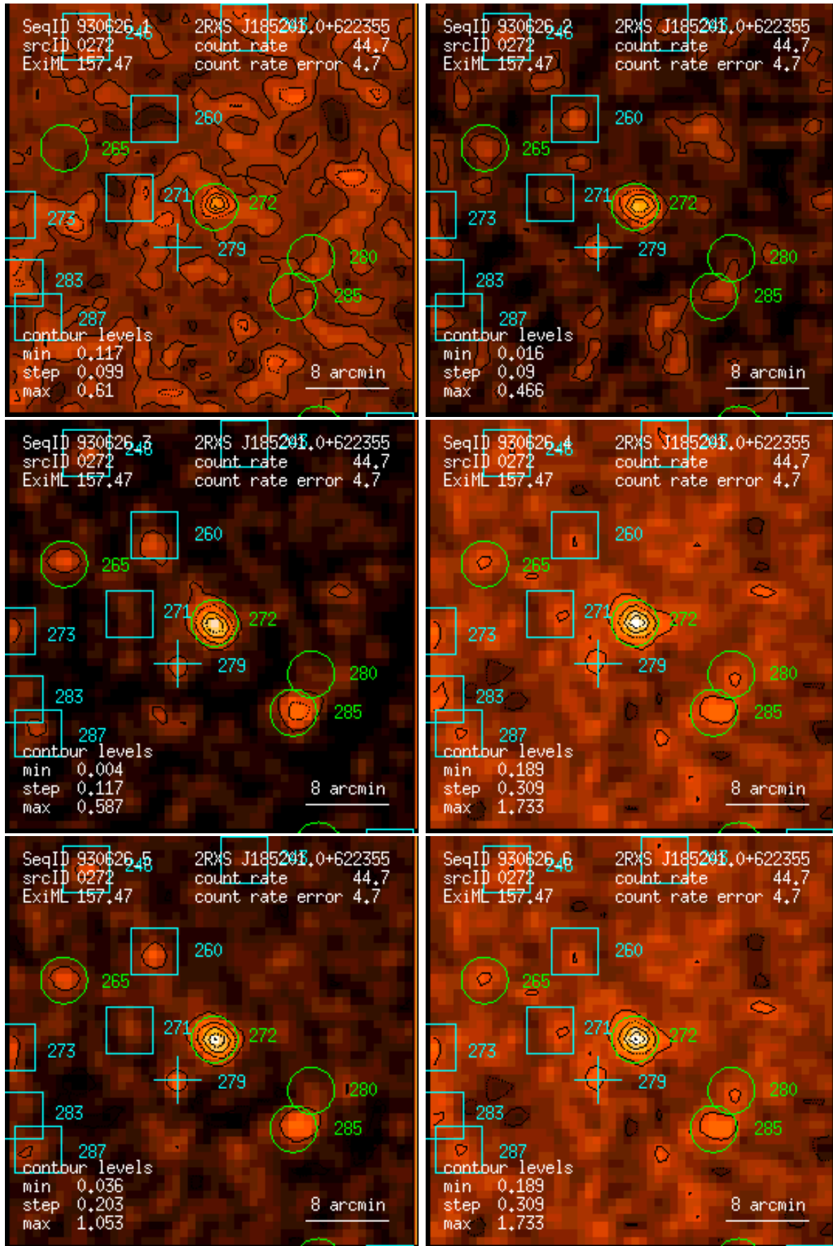
Figure 272: RASS 930626: detection 0272: band rate images, Gaussian filter: (1) PSPC channels 11 – 41, (2) 52 – 90, (3) 91 – 201, (4) 11 – 235, (5) 52 – 201, (6) 11 – 201. Broad band rates in counts/ks. Band rate contour levels in counts/ks/arcmin 2 .
