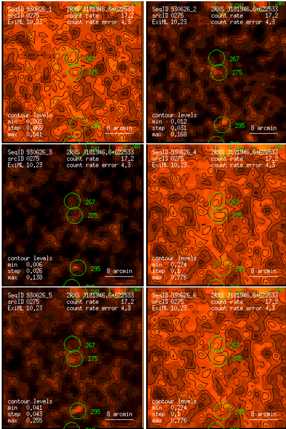
Figure 275: RASS 930626: detection 0275: band rate images, Gaussian filter: (1) PSPPC channels 11 – 41, (2) 52 – 90, (3) 91 – 201, (4) 11 – 235, (5) 52 – 201, (6) 11 – 201. Broad band rates in counts/ks. Band rate contour levels in counts/ks/arcmin 2 .
