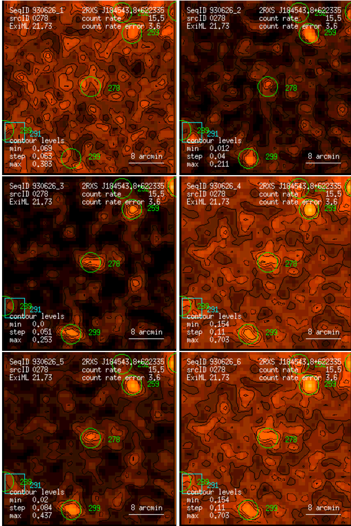
Figure 278: RASS 930626: detection 0278: band rate images, Gaussian filter: (1) PSPC channels 11 – 41, (2) 52 – 90, (3) 91 – 201, (4) 11 – 235, (5) 52 – 201, (6) 11 – 201. Broad band rates in counts/ks. Band rate contour levels in counts/ks/arcmin 2 .
