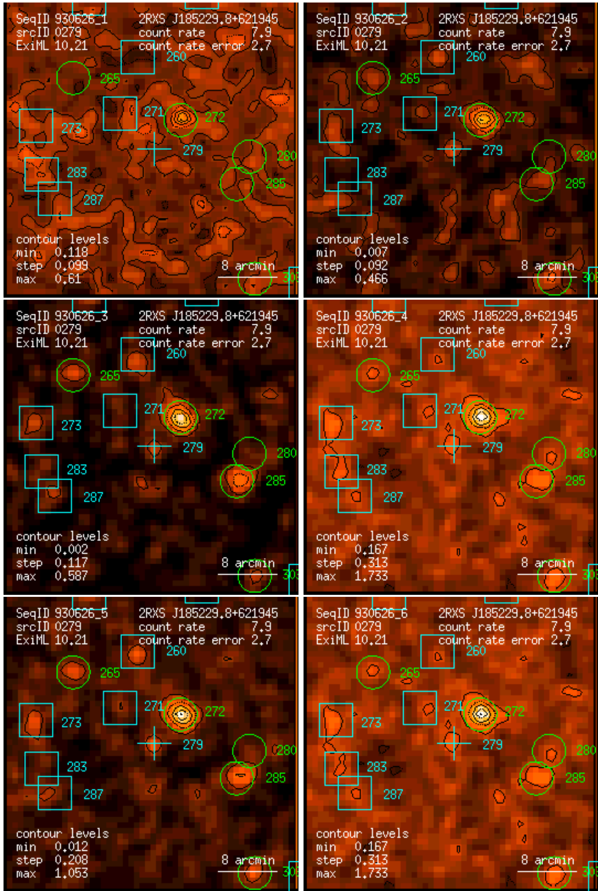
Figure 279: RASS 930626: detection 0279: band rate images, Gaussian filter: (1) PSPC channels 11 – 41, (2) 52 – 90, (3) 91 – 201, (4) 11 – 235, (5) 52 – 201, (6) 11 – 201. Broad band rates in counts/ks. Band rate contour levels in counts/ks/arcmin 2 .
