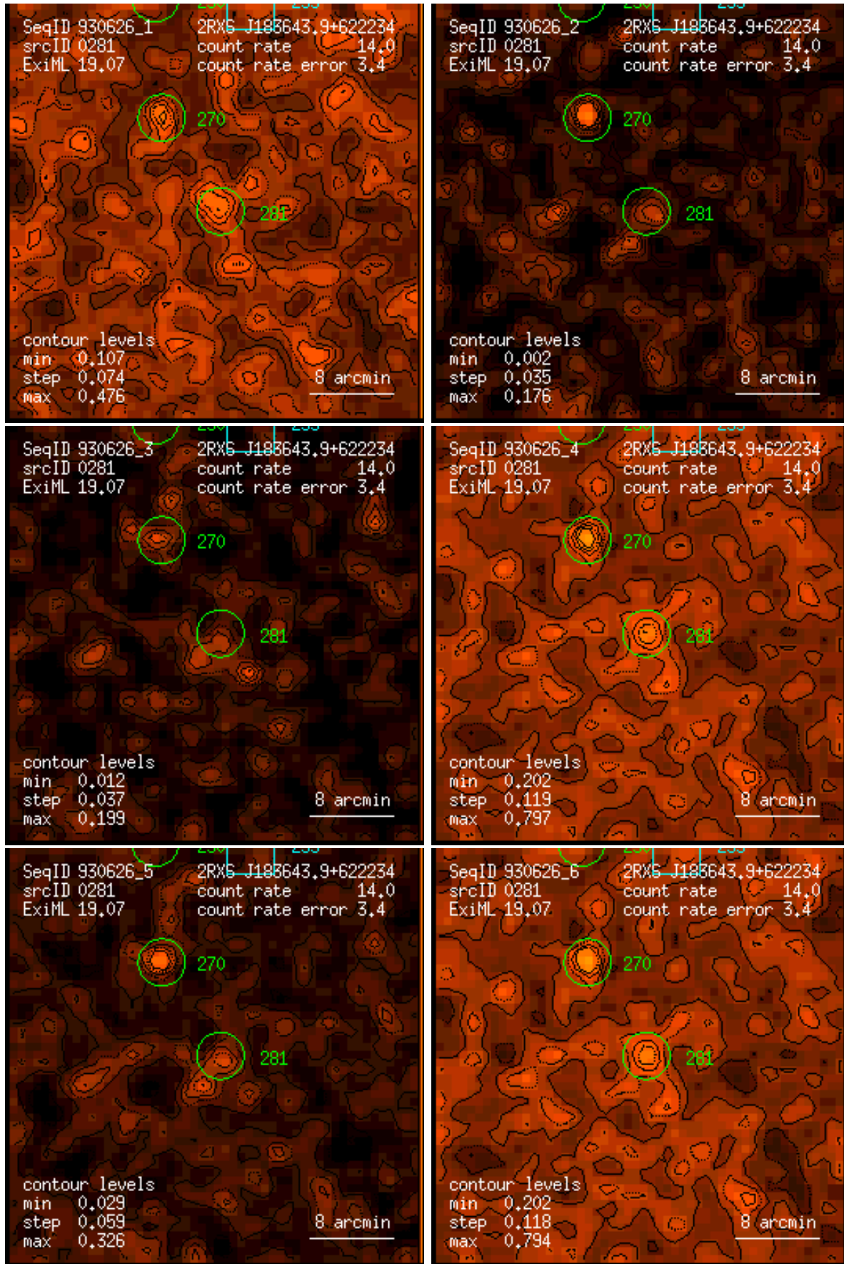
Figure 281: RASS 930626: detection 0281: band rate images, Gaussian filter: (1) PSPC channels 11 – 41, (2) 52 – 90, (3) 91 – 201, (4) 11 – 235, (5) 52 – 201, (6) 11 – 201. Broad band rates in counts/ks. Band rate contour levels in counts/ks/arcmin 2 .
