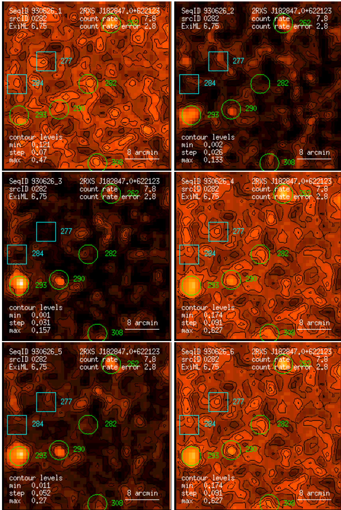
Figure 282: RASS 930626: detection 0282: band rate images, Gaussian filter: (1) PSPC channels 11 – 41, (2) 52 – 90, (3) 91 – 201, (4) 11 – 235, (5) 52 – 201, (6) 11 – 201. Broad band rates in counts/ks. Band rate contour levels in counts/ks/arcmin 2 .
