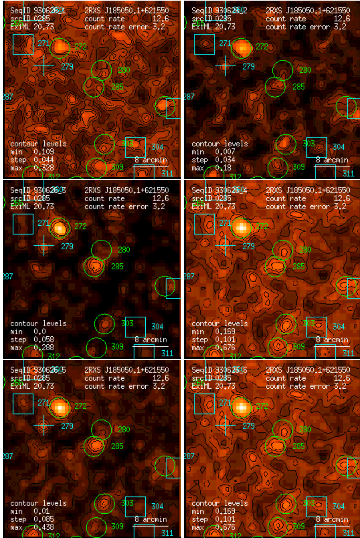
Figure 285: RASS 930626: detection 0285: band rate images, Gaussian filter: (1) PSPC channels 11 – 41, (2) 52 – 90, (3) 91 – 201, (4) 11 – 235, (5) 52 – 201, (6) 11 – 201. Broad band rates in counts/ks. Band rate contour levels in counts/ks/arcmin 2 .
