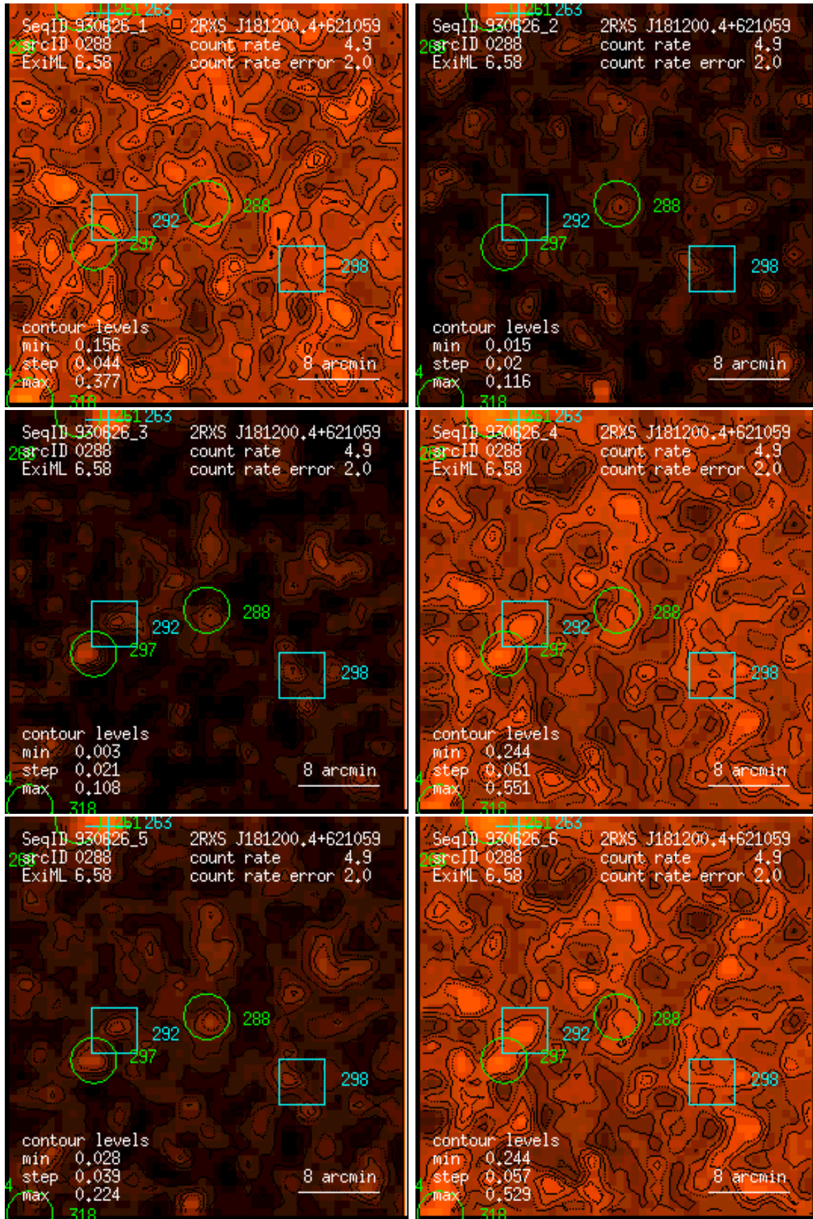
Figure 288: RASS 930626: detection 0288: band rate images, Gaussian filter: (1) PSPC channels 11 – 41, (2) 52 – 90, (3) 91 – 201, (4) 11 – 235, (5) 52 – 201, (6) 11 – 201. Broad band rates in counts/ks. Band rate contour levels in counts/ks/arcmin 2 .
