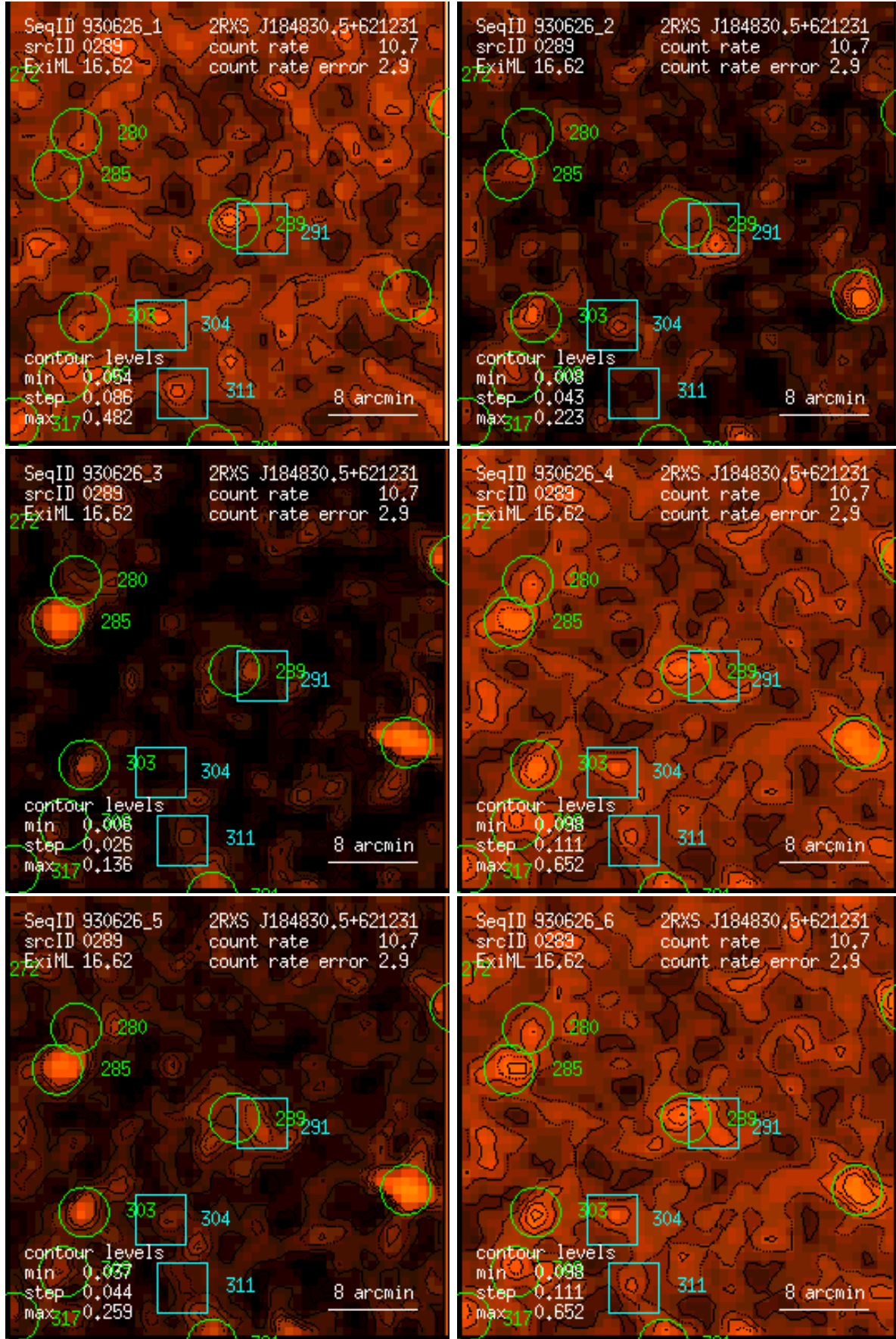
Figure 289: RASS 930626: detection 0289: band rate images, Gaussian filter: (1) PSPC channels 11 – 41, (2) 52 – 90, (3) 91 – 201, (4) 11 – 235, (5) 52 – 201, (6) 11 – 201. Broad band rates in counts/ks. Band rate contour levels in counts/ks/arcmin 2 .
