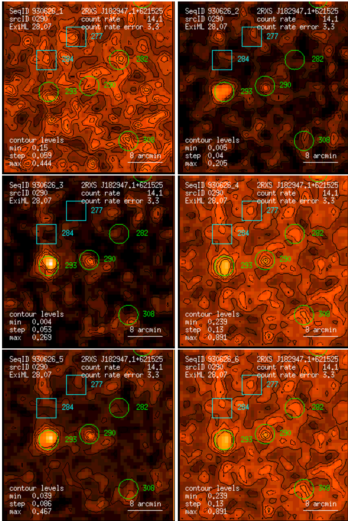
Figure 290: RASS 930626: detection 0290: band rate images, Gaussian filter: (1) PSPC channels 11 – 41, (2) 52 – 90, (3) 91 – 201, (4) 11 – 235, (5) 52 – 201, (6) 11 – 201. Broad band rates in counts/ks. Band rate contour levels in counts/ks/arcmin 2 .
