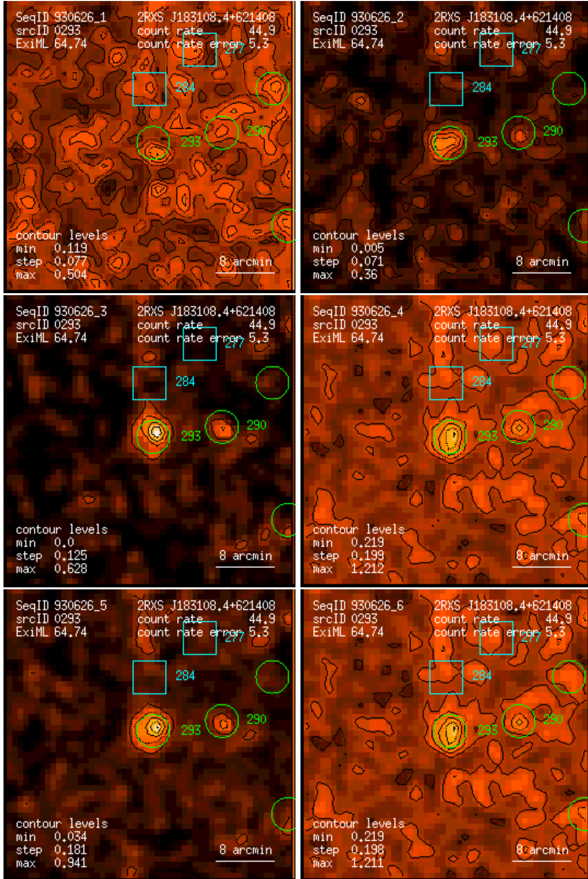
Figure 293: RASS 930626: detection 0293: band rate images, Gaussian filter: (1) PSPC channels 11 – 41, (2) 52 – 90, (3) 91 – 201, (4) 11 – 235, (5) 52 – 201, (6) 11 – 201. Broad band rates in counts/ks. Band rate contour levels in counts/ks/arcmin 2 .
