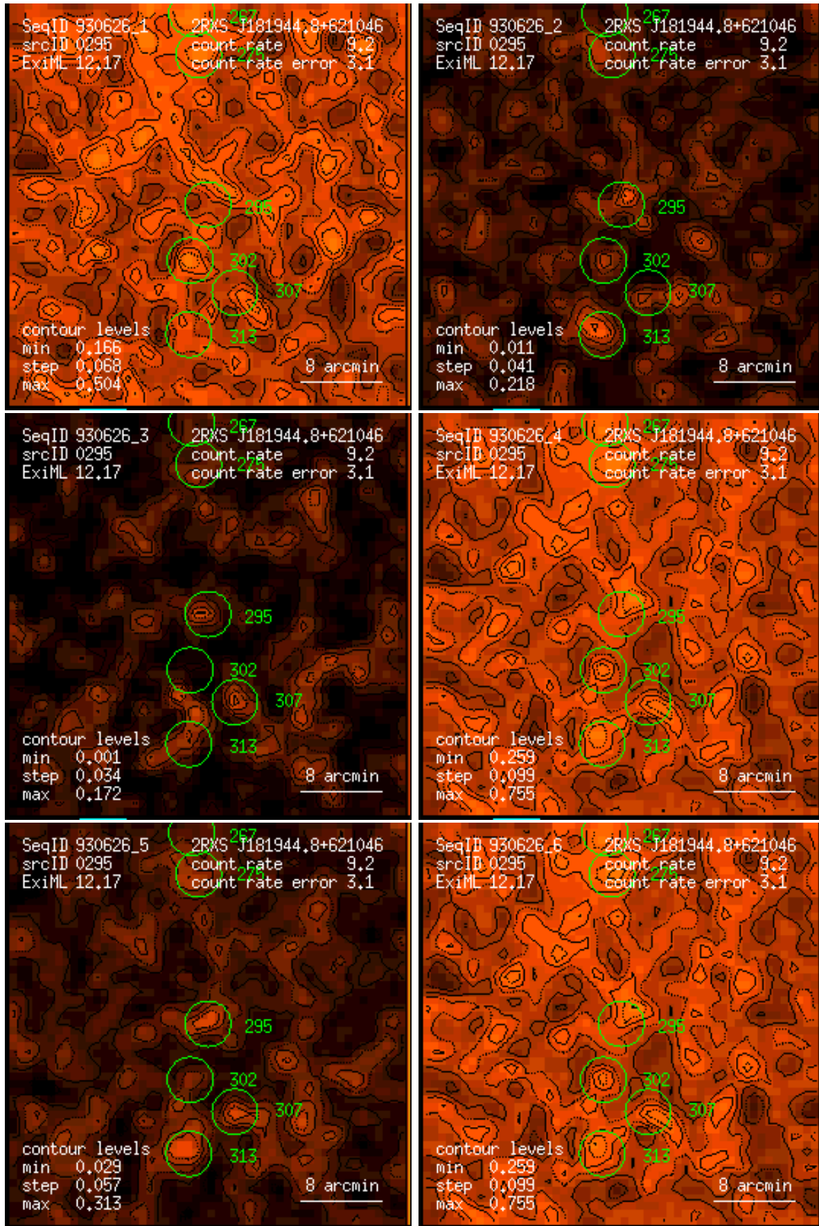
Figure 295: RASS 930626: detection 0295: band rate images, Gaussian filter: (1) PSPC channels 11 – 41, (2) 52 – 90, (3) 91 – 201, (4) 11 – 235, (5) 52 – 201, (6) 11 – 201. Broad band rates in counts/ks. Band rate contour levels in counts/ks/arcmin 2 .
