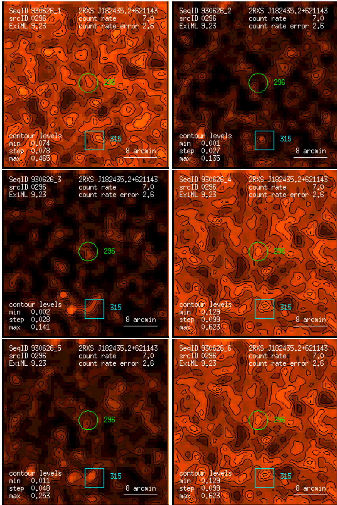
Figure 296: RASS 930626: detection 0296: band rate images, Gaussian filter: (1) PSPC channels 11 – 41, (2) 52 – 90, (3) 91 – 201, (4) 11 – 235, (5) 52 – 201, (6) 11 – 201. Broad band rates in counts/ks. Band rate contour levels in counts/ks/arcmin 2 .
