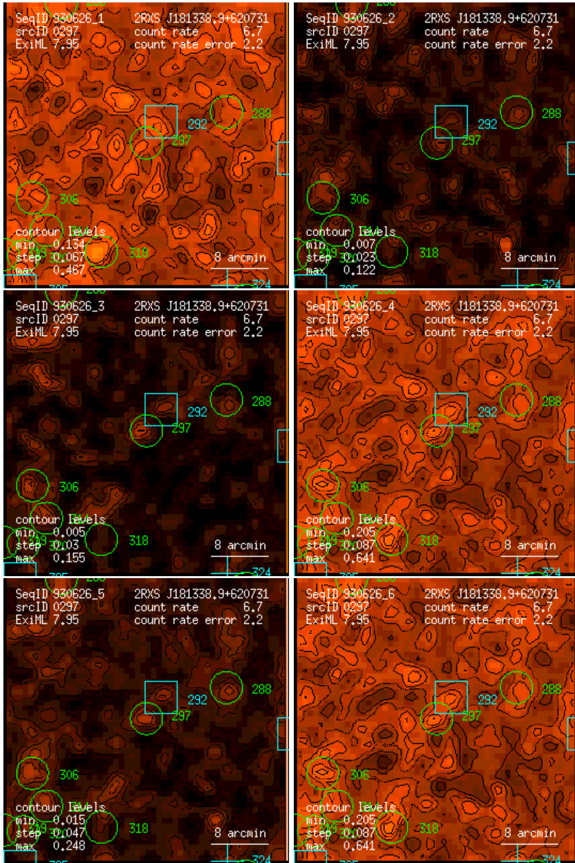
Figure 297: RASS 930626: detection 0297: band rate images, Gaussian filter: (1) PSPC channels 11 – 41, (2) 52 – 90, (3) 91 – 201, (4) 11 – 235, (5) 52 – 201, (6) 11 – 201. Broad band rates in counts/ks. Band rate contour levels in counts/ks/arcmin 2 .
