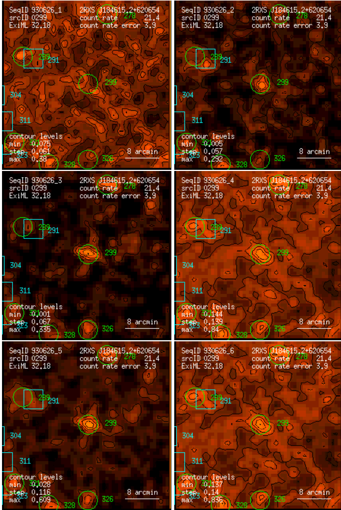
Figure 299: RASS 930626: detection 0299: band rate images, Gaussian filter: (1) PSPC channels 11 – 41, (2) 52 – 90, (3) 91 – 201, (4) 11 – 235, (5) 52 – 201, (6) 11 – 201. Broad band rates in counts/ks. Band rate contour levels in counts/ks/arcmin 2 .
